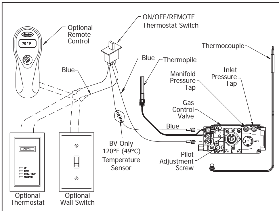
Figure 32: Accessory Wiring
