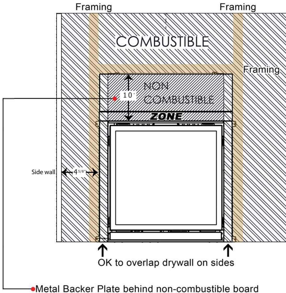
Figure 18B. Non Combustable Material
