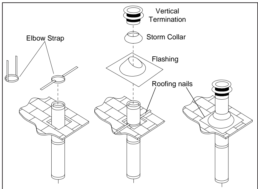
Figure 26A. Vertical Vent Termination
