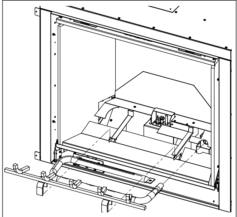
Figure 10. Removing Burner
