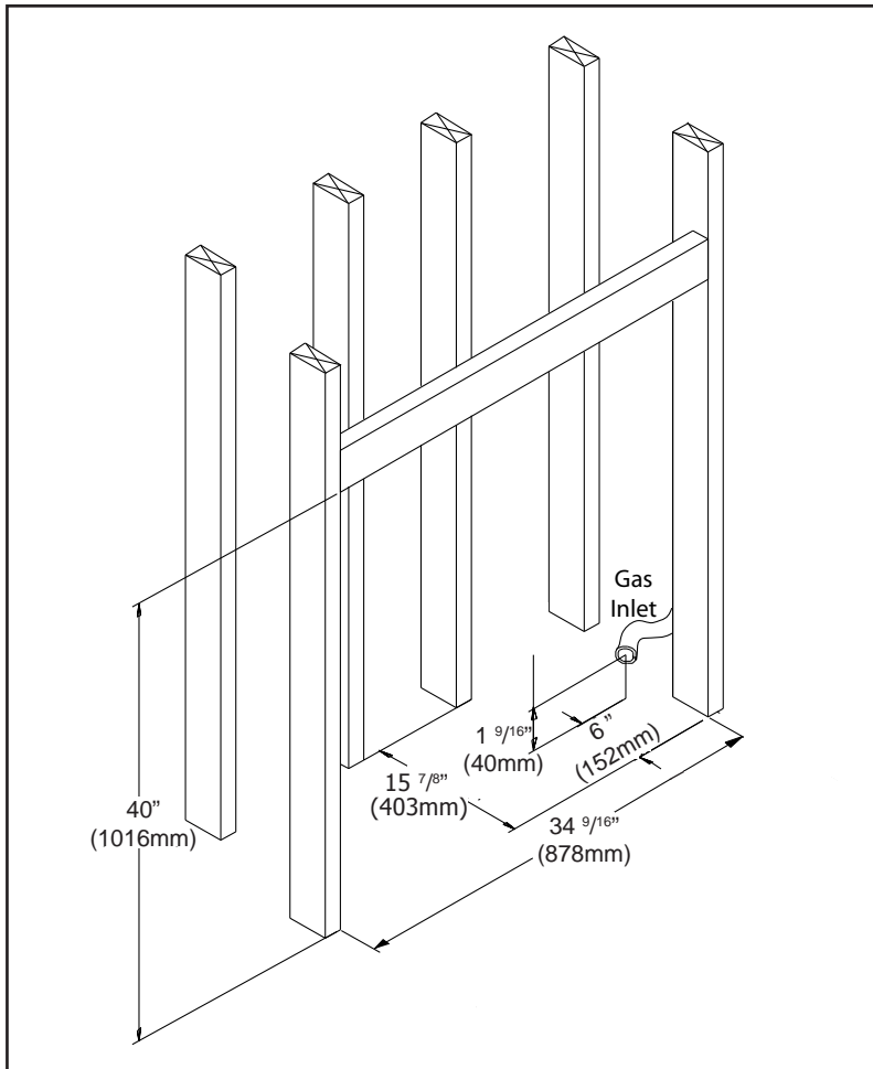
Figure 12. Dimensions for Framing the Firebox
