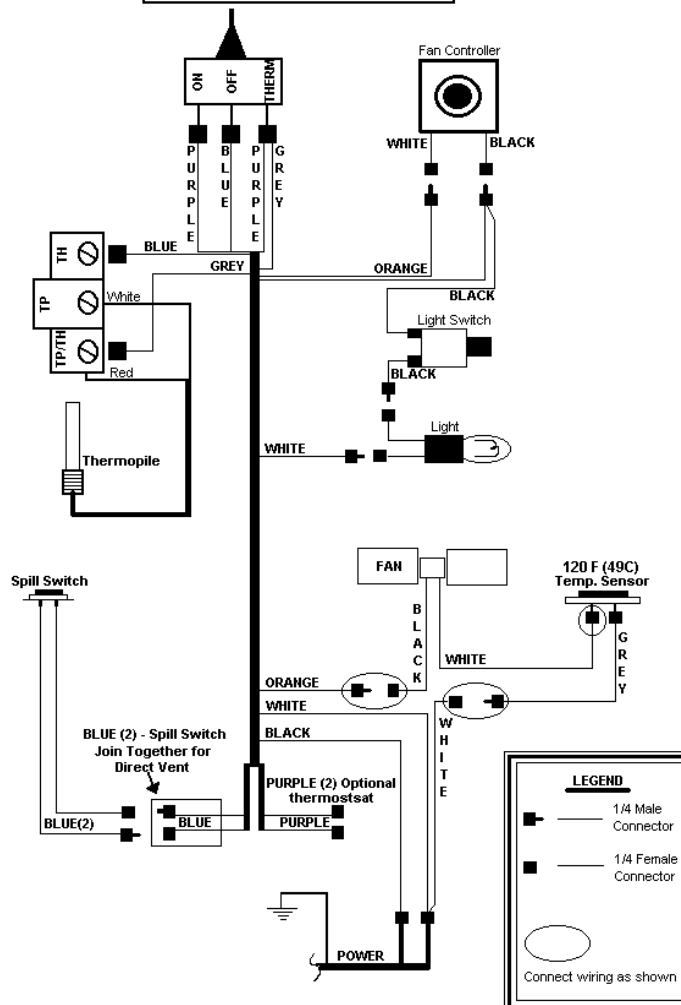
ENVIROGAS-28 Wiring Diagram
