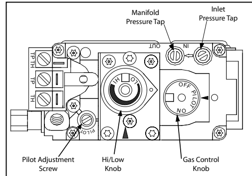
Figure 37: Fully Labeled Gas Valve.
