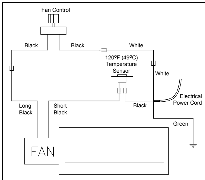
Figure 38. Wiring Diagram For Fan Control.
