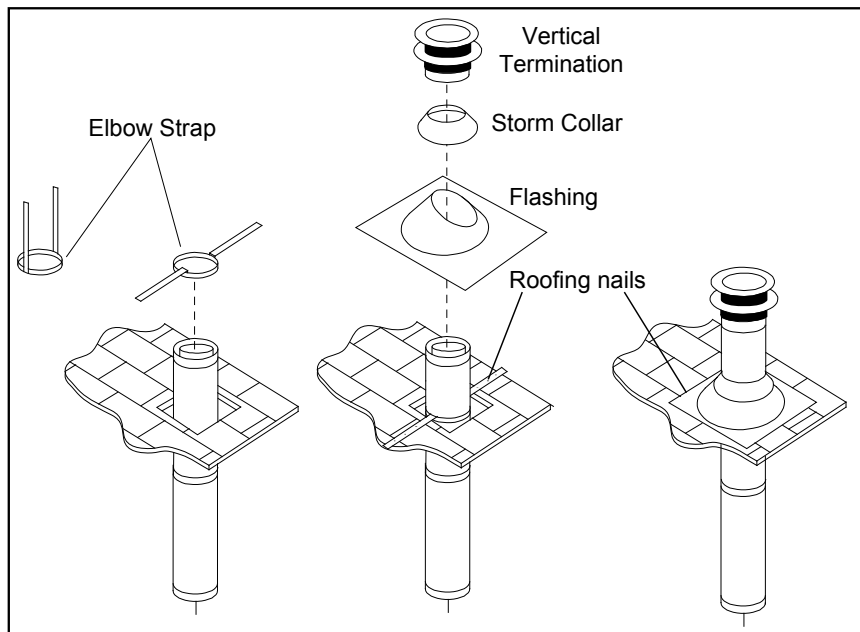
Figure 31. Vertical Vent Termination
