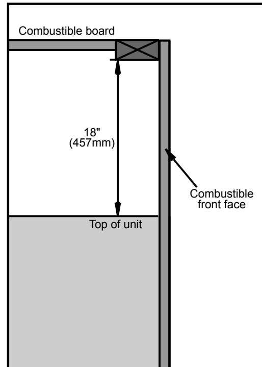
Figure 21. Combustible Shelf Clearance.
