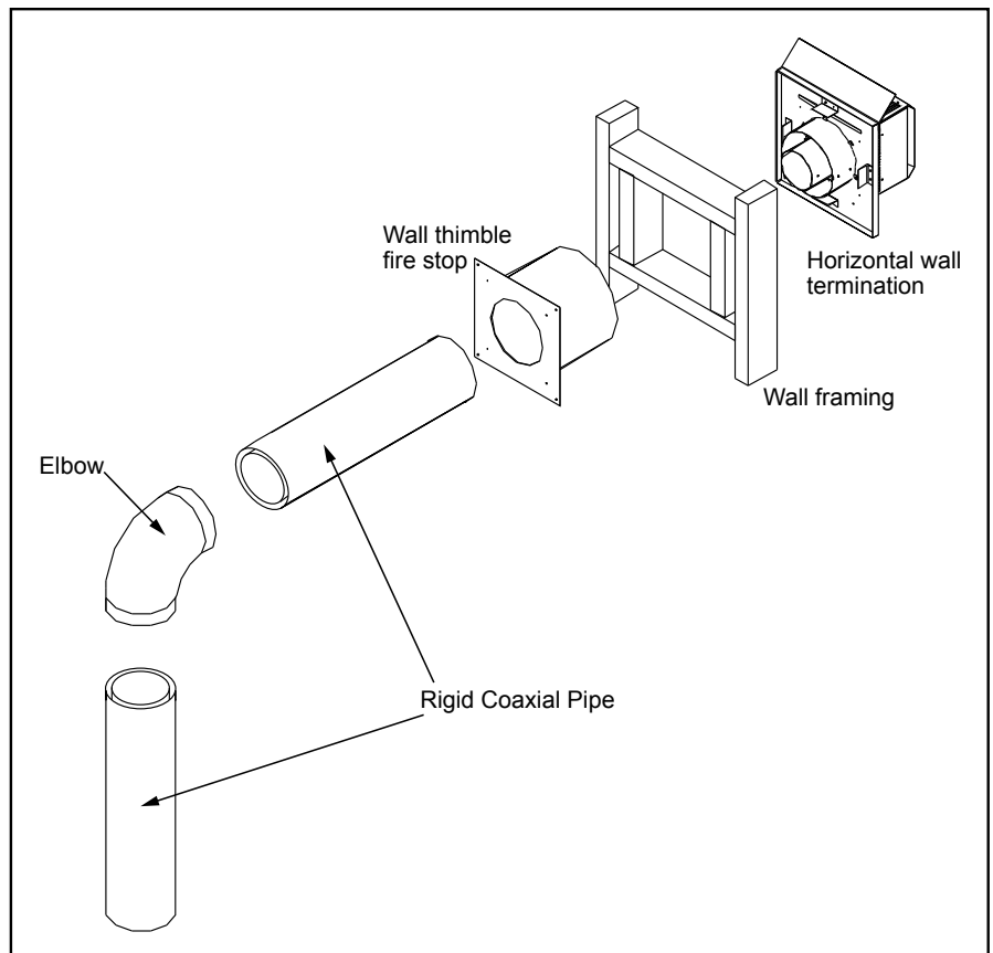
Figure 30. Horizontal Vent Termination
