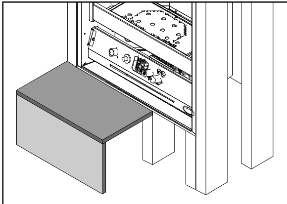
Figure 12. Raised Fireplace with Raised Hearth.
