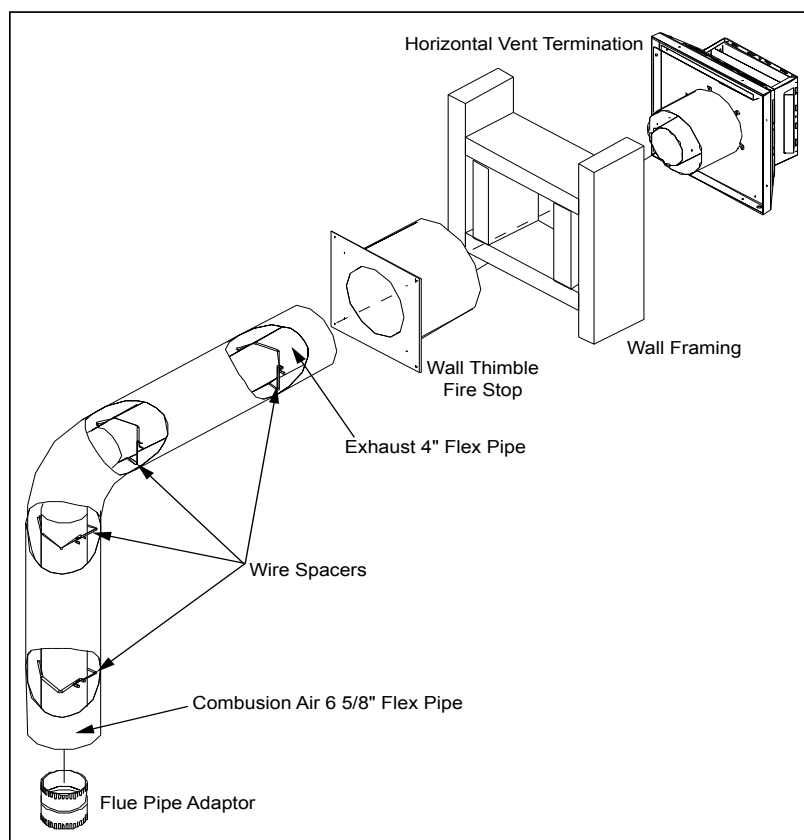
Figure 25: Installation of Fireplace Horizontal Vent Kit.
