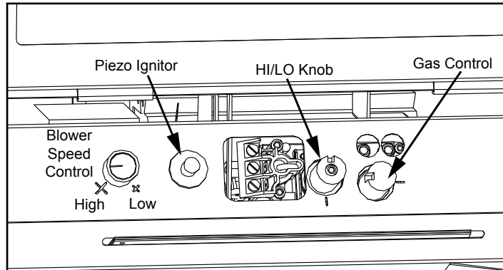
Figure 5. Control Panel
