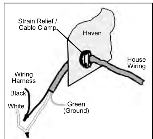
Figure 36. Install Electrical 14/2 Wire Power Cable Into Haven.
