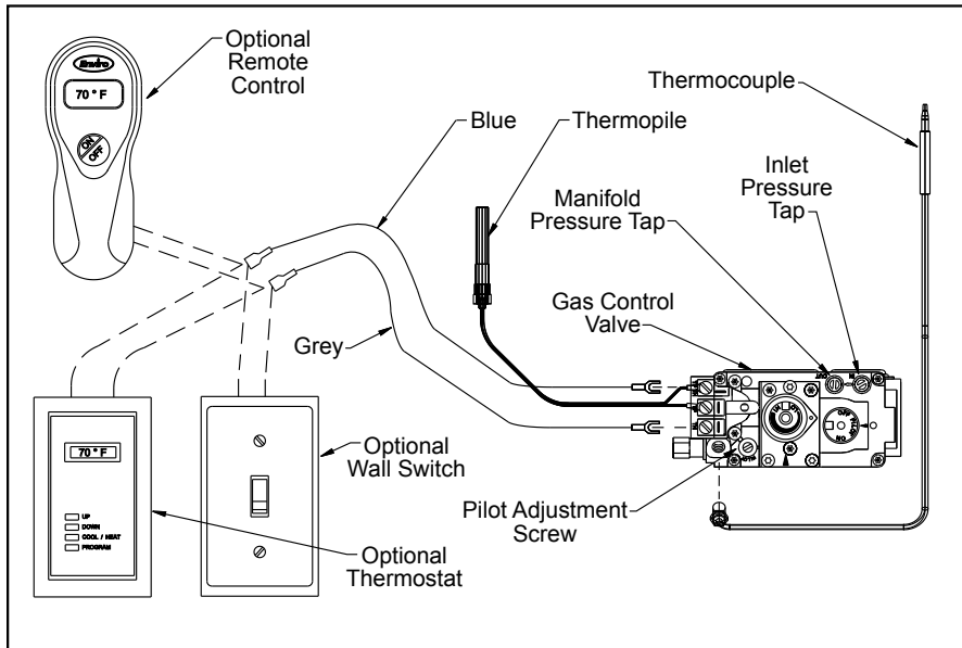
Figure 35. Wiring Diagram For Gas Valve.
