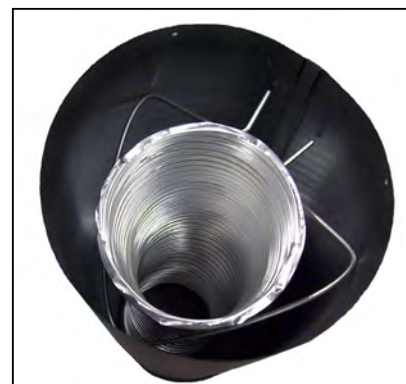
Figure 24: Wire Spacer in Place.
