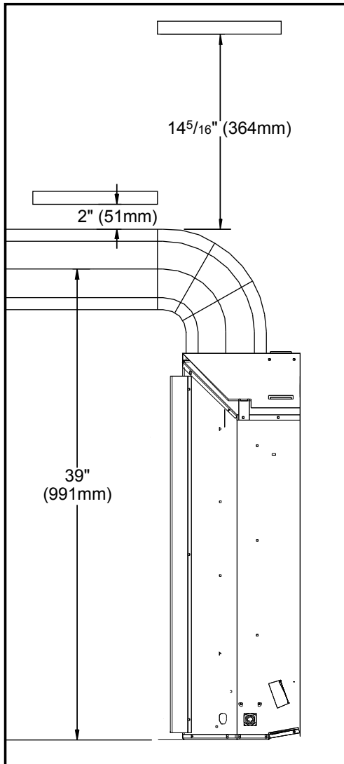
Figure 26. Vent Pipe Clearances.
