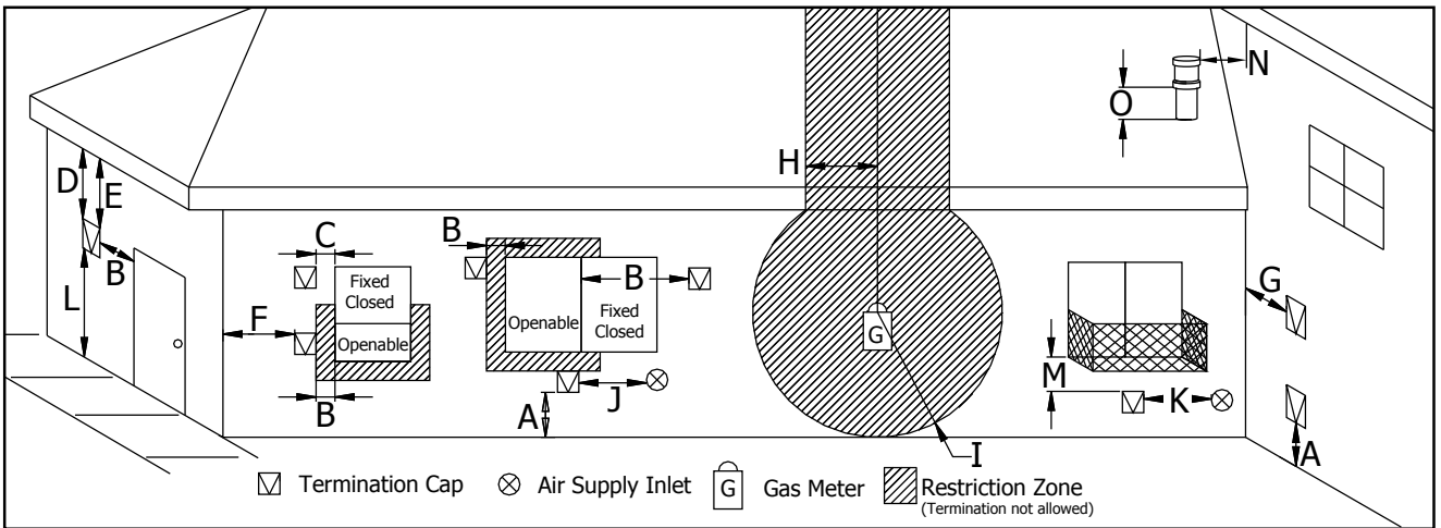
Figure 22. Vent Termination Restrictions, refer to Table 3.
