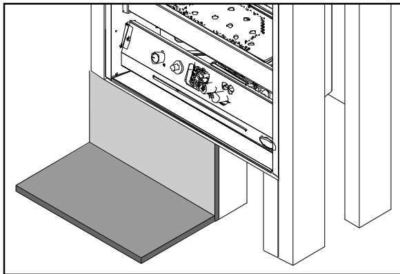
Figure 12. Raised Fireplace with Floor Level Hearth.
