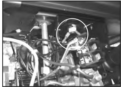
Figure 42: Installing Temperature Sensor.
