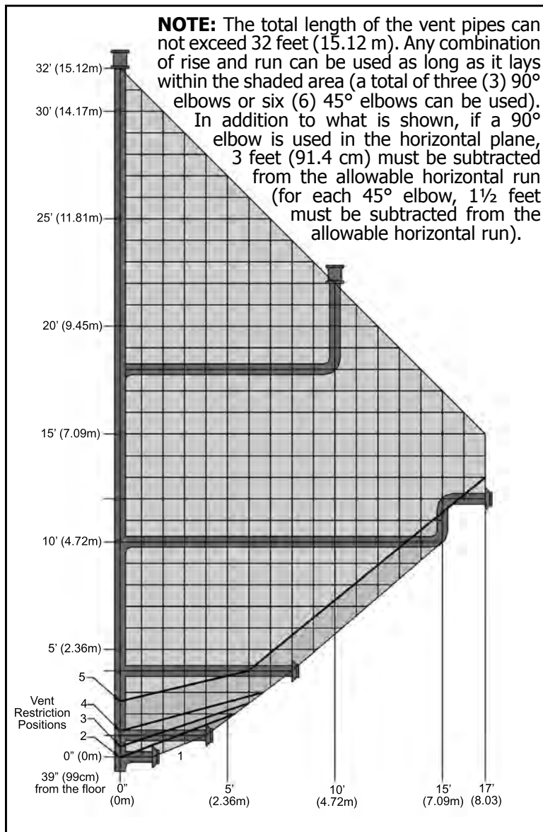
Figure 28. Possible Vent Configurations for Top Vented; Vertical and Horizontal Terminations.
