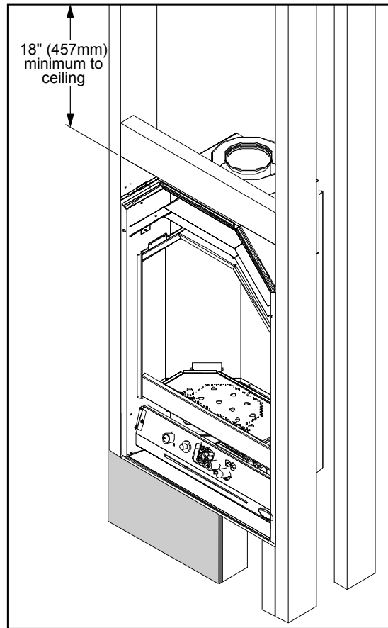
Figure 14. Raised Fireplace with No Hearth.
