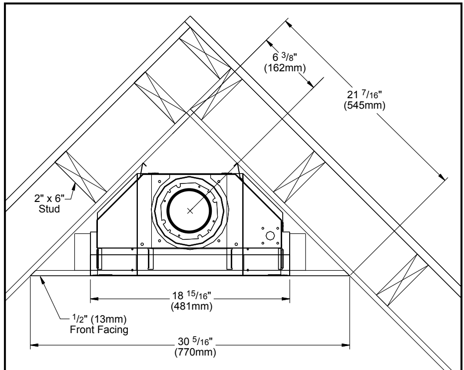
Figure 11. Dimensions for a corner installation.
