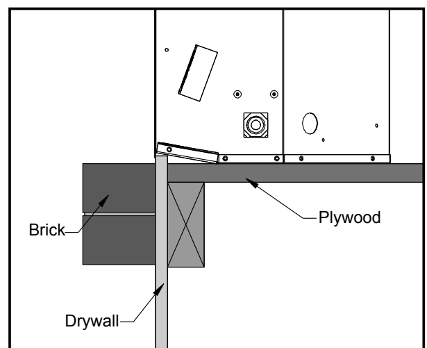
Figure 19. Drywall & Brick Facing Around The Haven.
