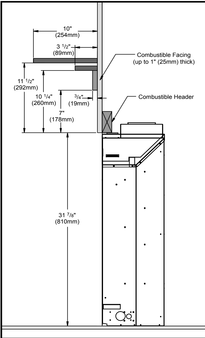
Figure 20. Combustible Mantle Clearances.
