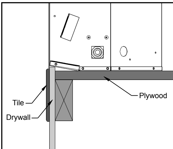
Figure 18. Drywall & Tile Facing Around The Haven.
