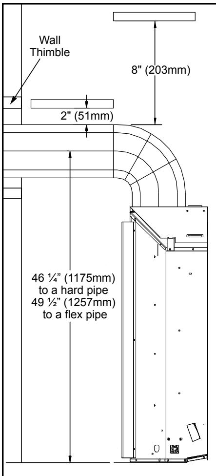
Figure 29. Vent Pipe Clearances.
