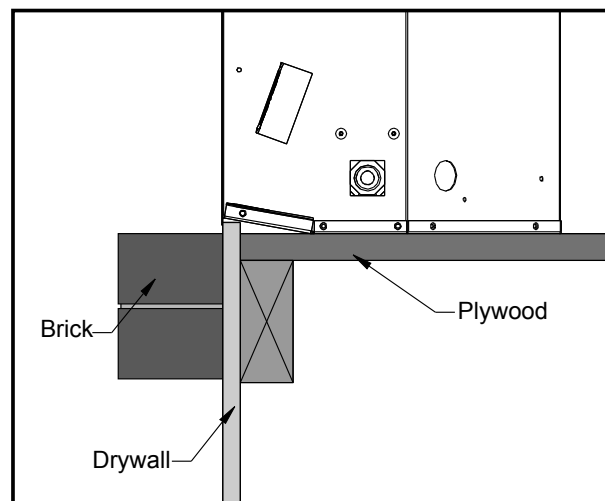
Figure 22. Drywall & Brick Facing Around The Retreat.
