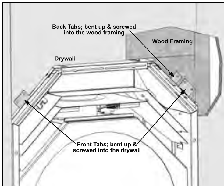
Figure 18. Top Mounting brackets.
