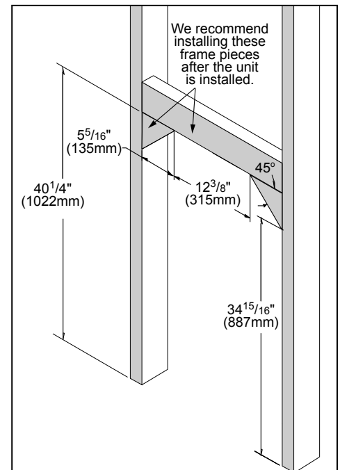
Figure 13. Dimensions for Top Framing the Firebox.
