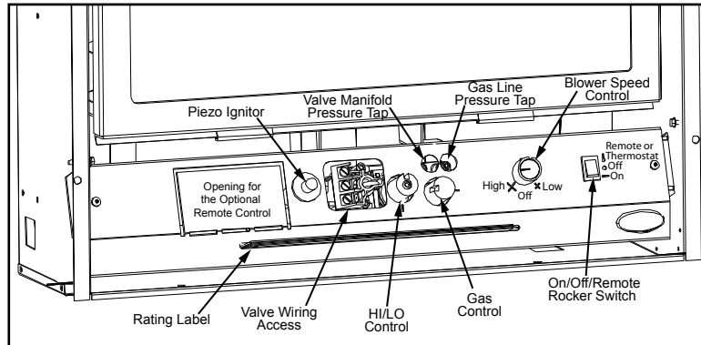
Figure 5. Control Panel
