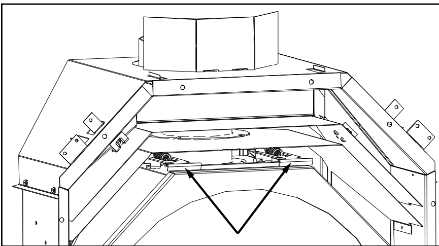
Figure 7. Top latches for glass door, engaged.
