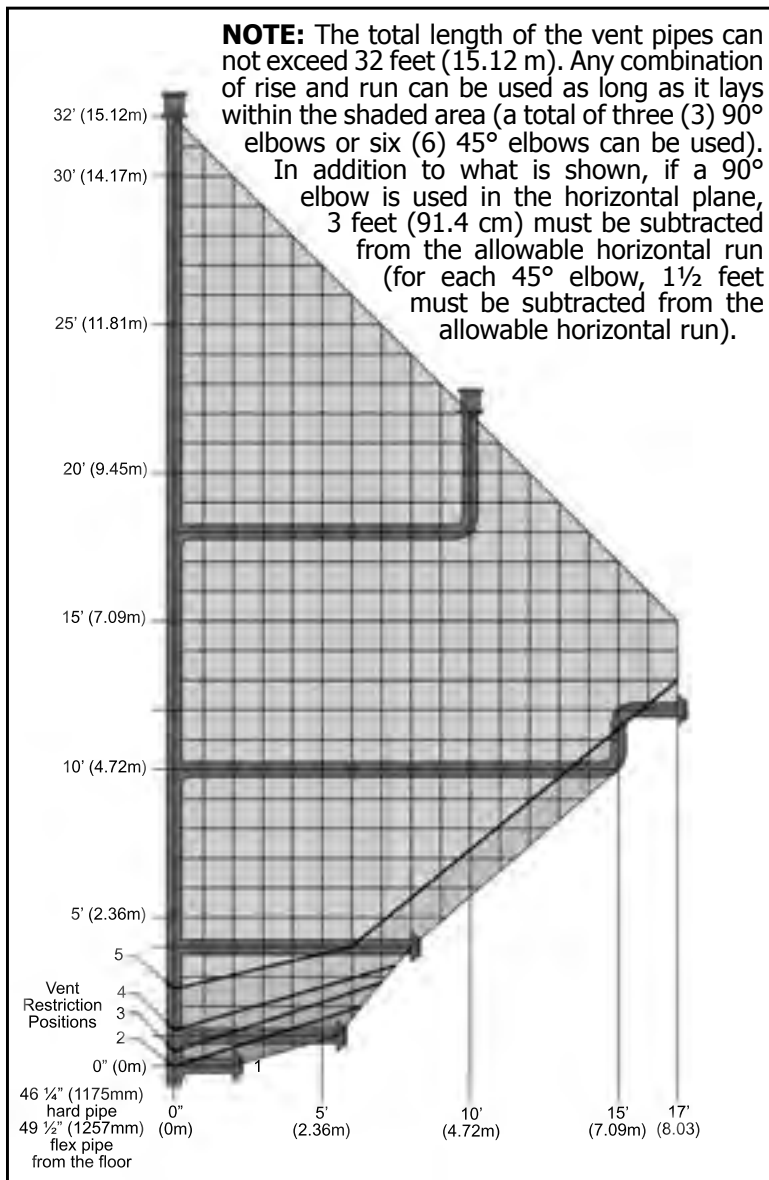
Figure 31. Possible Vent Configurations for Top Venting; Vertical and Horizontal Terminations.
