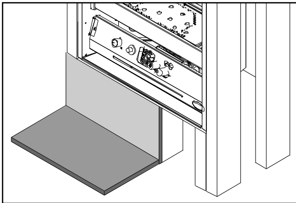
Figure 16. Raised Fireplace with Floor Level Hearth.
