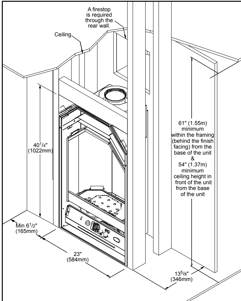
Figure 12. Dimensions for Framing the Firebox.
