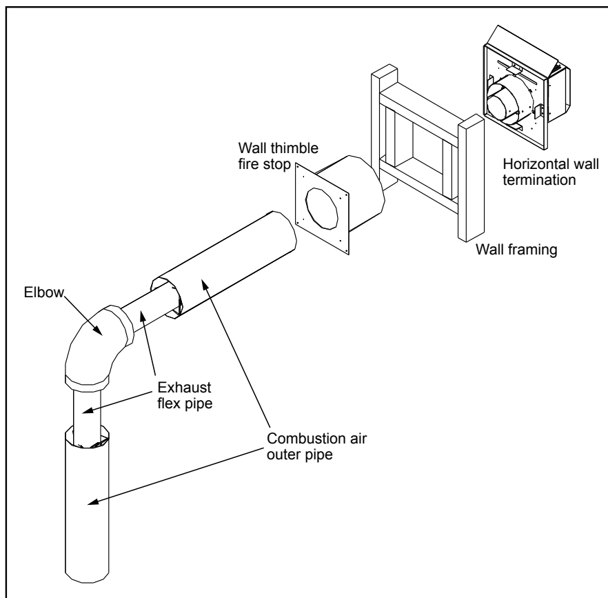
Figure 25. Horizontal Vent Termination
