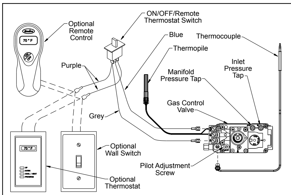
Figure 34. Wiring Diagram For Gas Valve.
