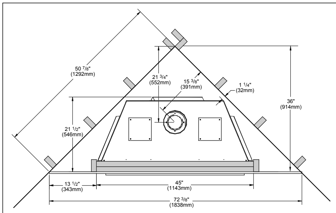
Figure 11. Dimensions for a corner installation.
