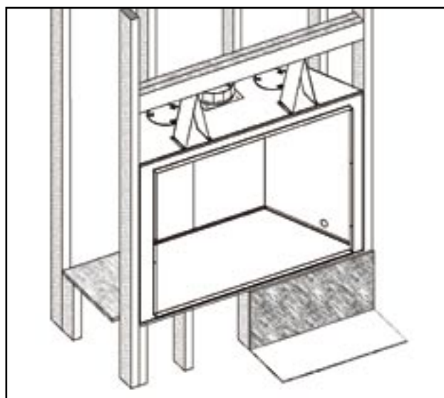
Figure 13. Raised Fireplace with Floor Level Hearth
