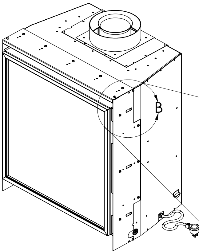
Figure 28: Position of Extension Brackets at biggest depth
