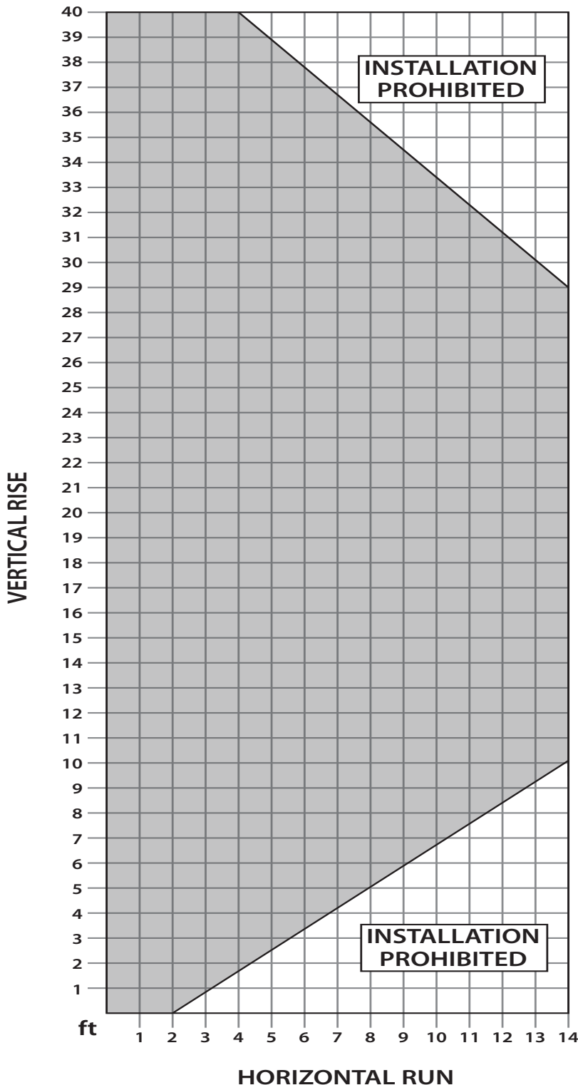
Figure 35. Possible Vent Configurations for Top Vented Vertical and Horizontal Terminations.
