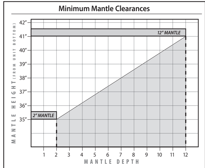
Figure 30. Mantle Clearances
