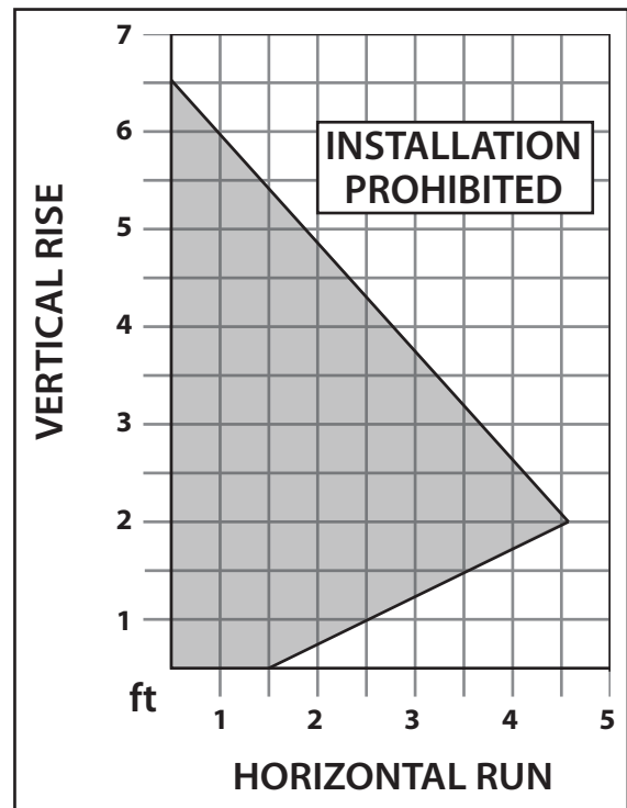
Figure 36. Possible Vent Configurations for Rear Vented Vertical and Horizontal Terminations.
