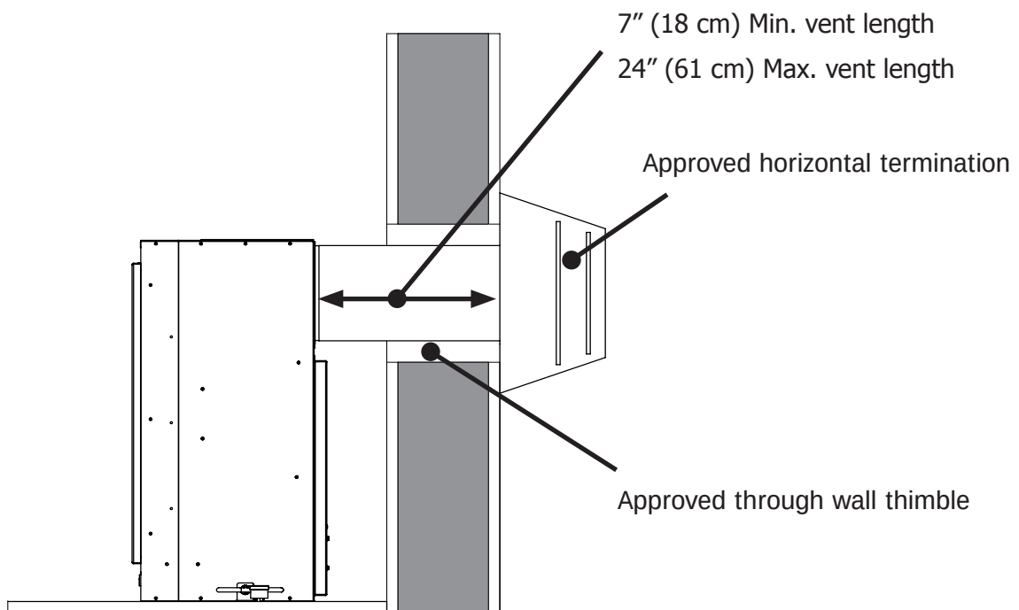
Figure 34. Flat to Wall Rear Vent - No Vertical Rise
