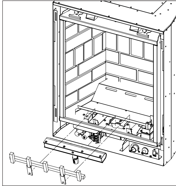
Figure 10. Removing Burner.
