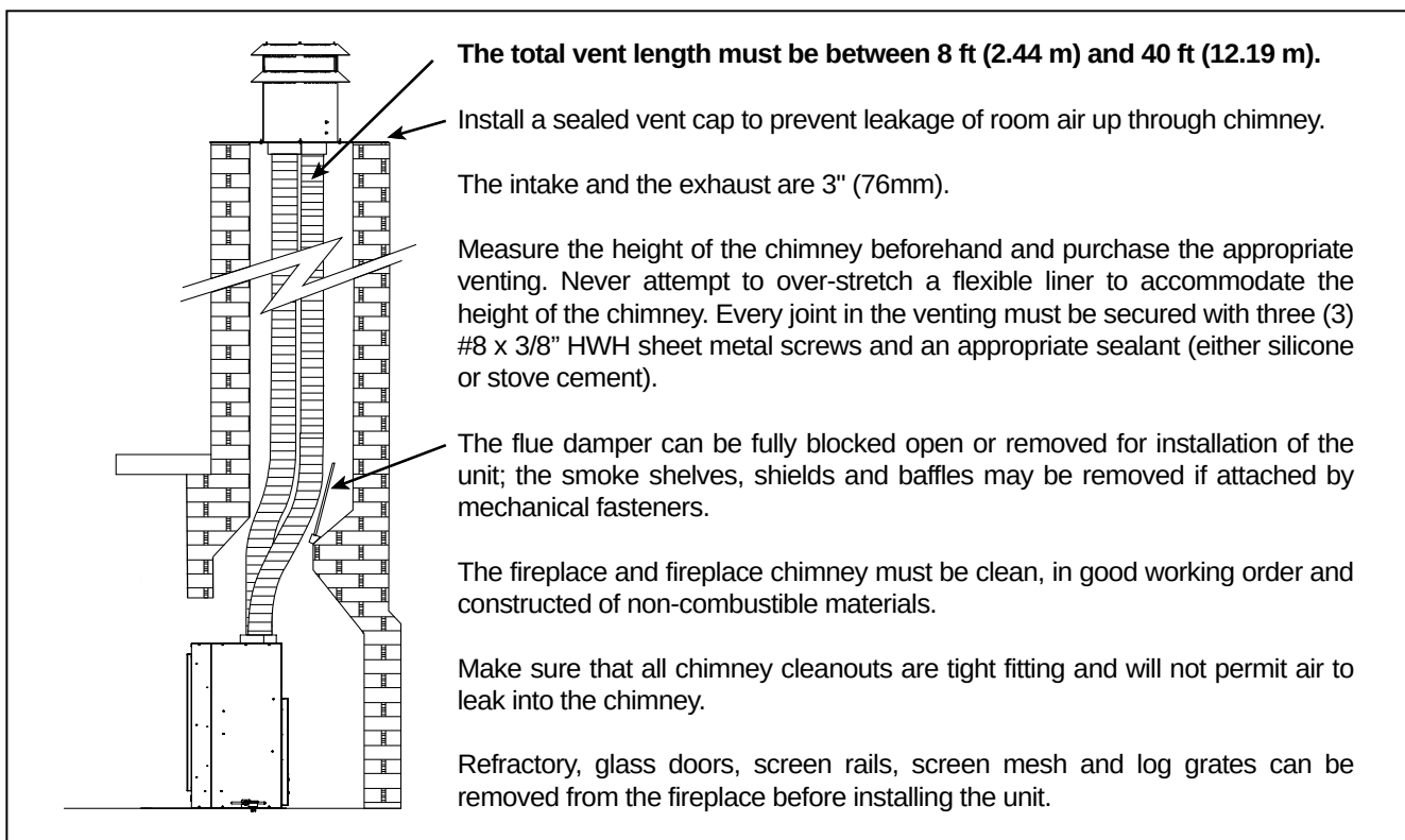
Figure 47: Solid Fuel Fireplace Installation.
