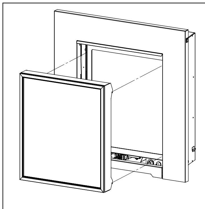
Figure 64: Installing Safety Screen onto Brackets.
