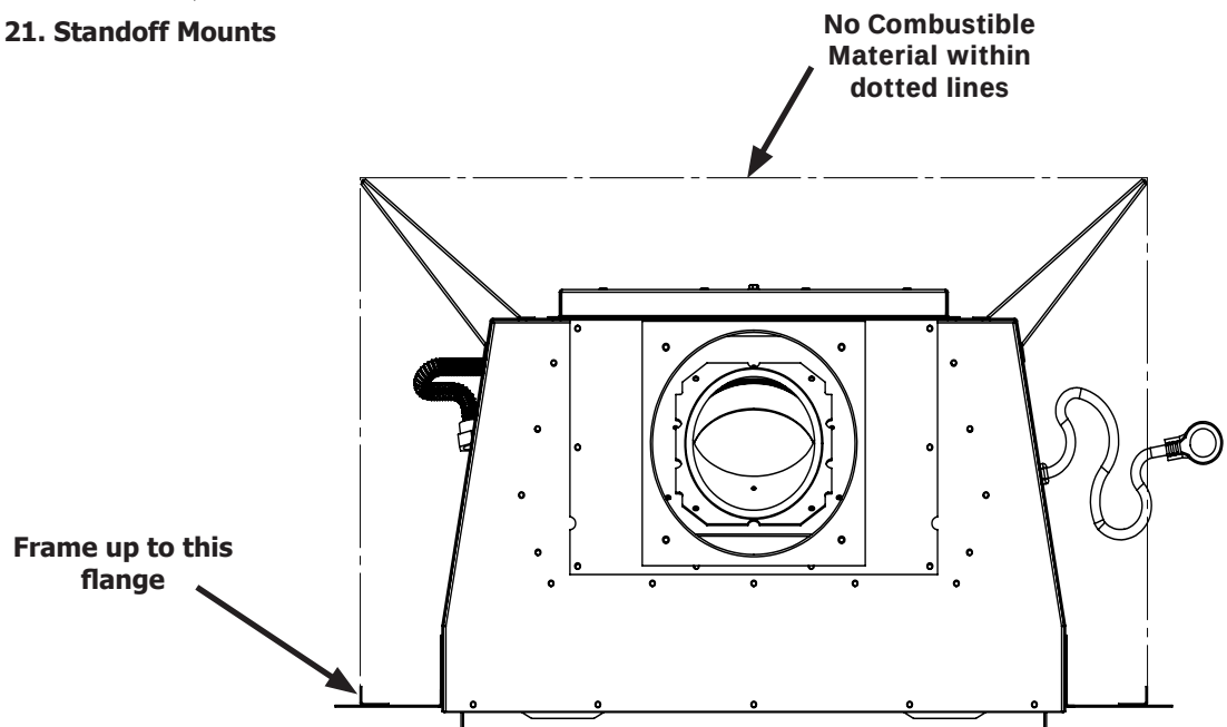
Figure 22. Area created by standoffs
