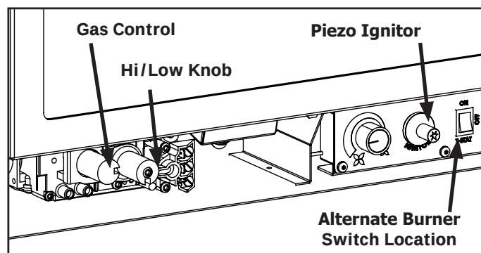
Figure 6. Control Panel
