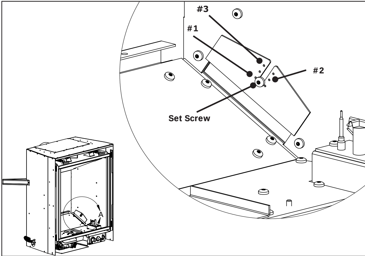
Figure 41: Installation of Air Restrictors
