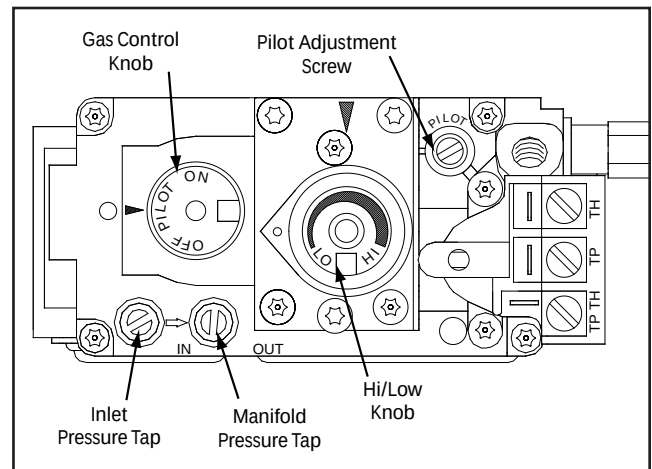
Figure 49: Fully Labeled Gas Valve.
