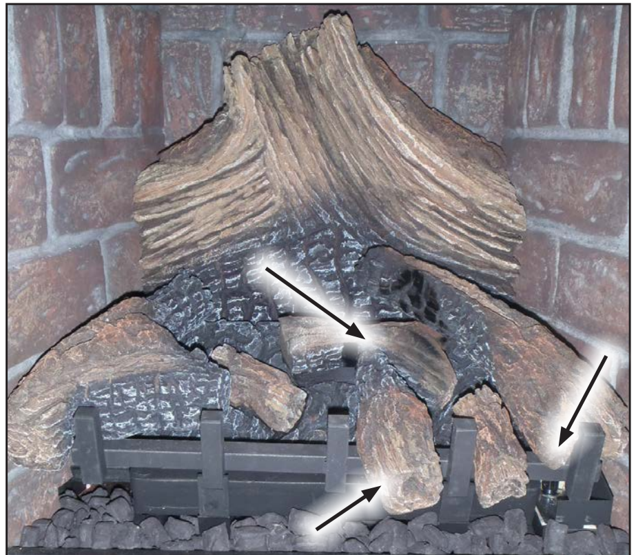
Figure 56. Fourth Stage Log Set Installation.
