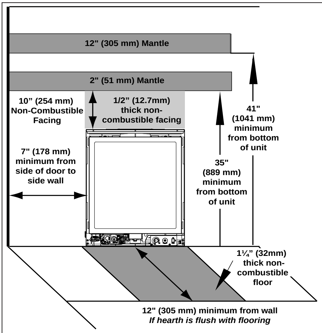
Figure 29. Non-Combustible Clearances
