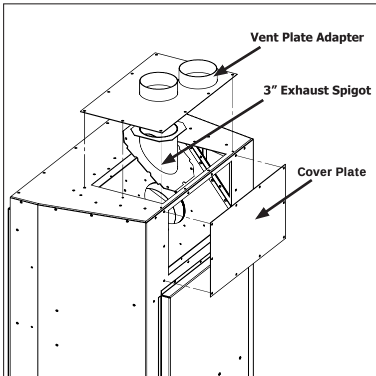
Figure 40: Installation of Co-Linear Vent Kit
