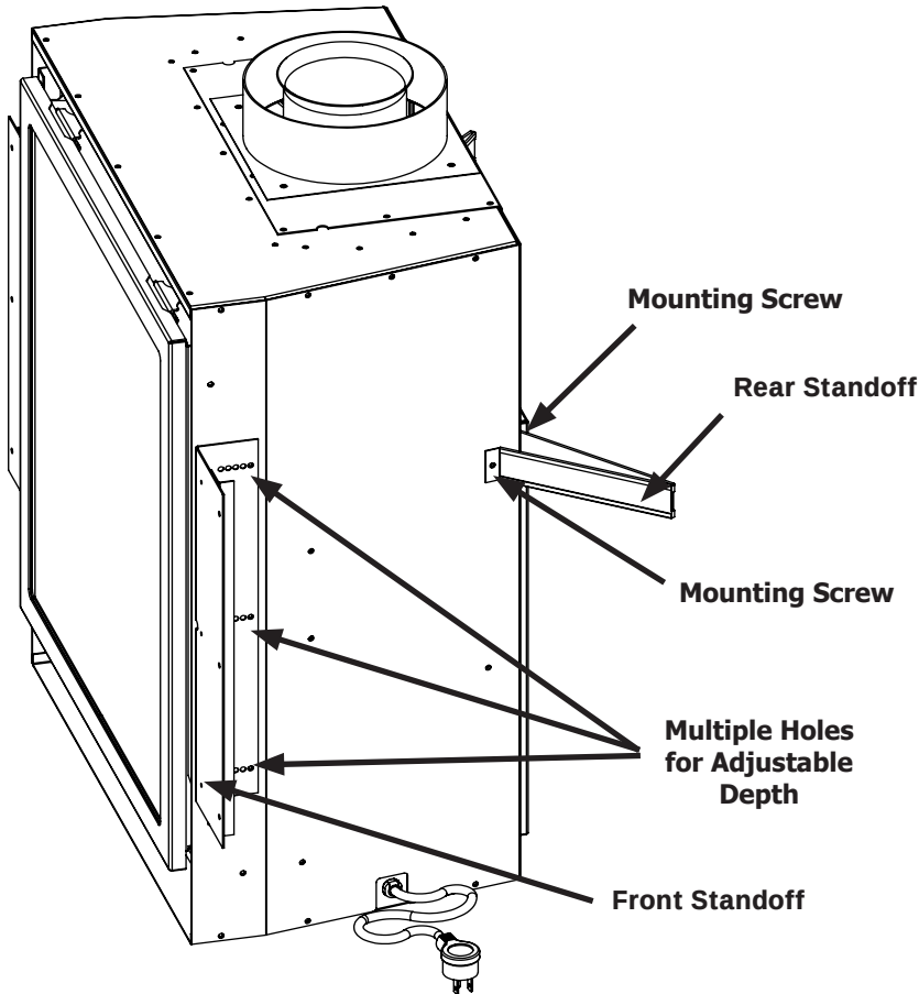
Figure 21. Standoff Mounts
