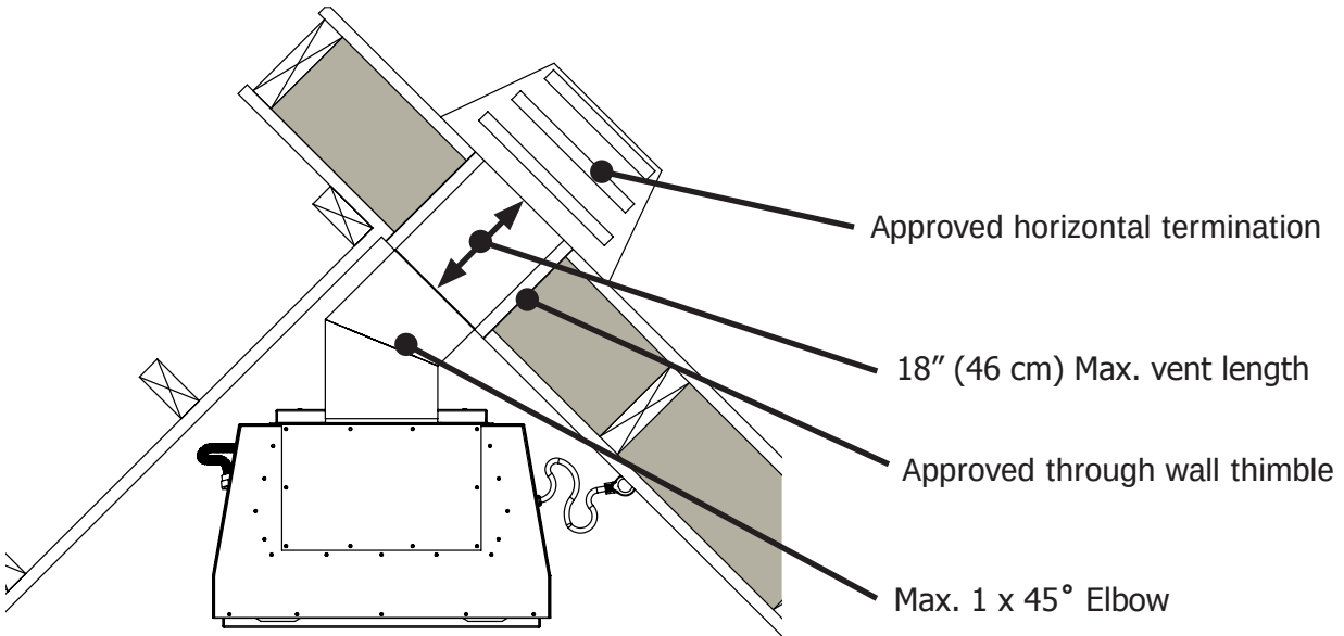
Figure 33. Corner Rear Vent - No Vertical Rise
