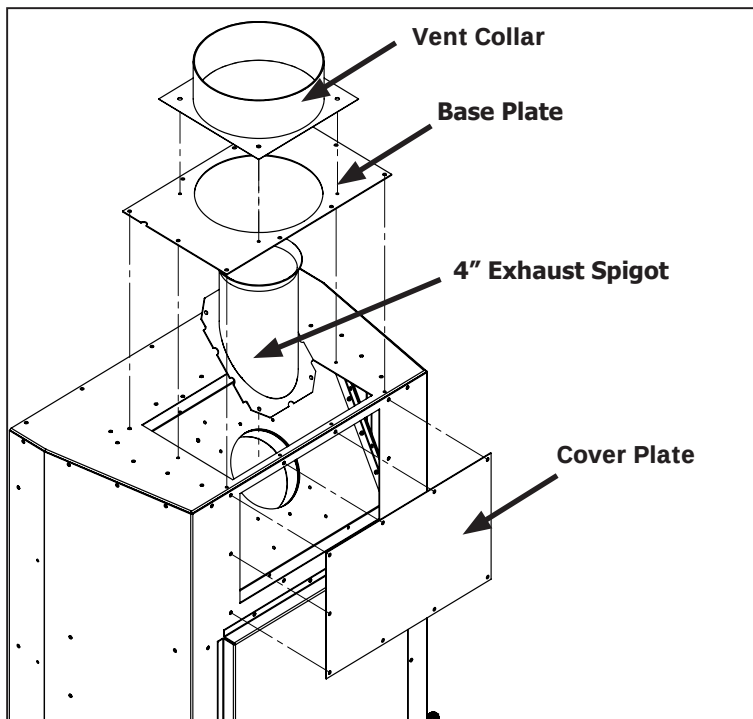
Figure 39: Removal of Co-Axial Venting
