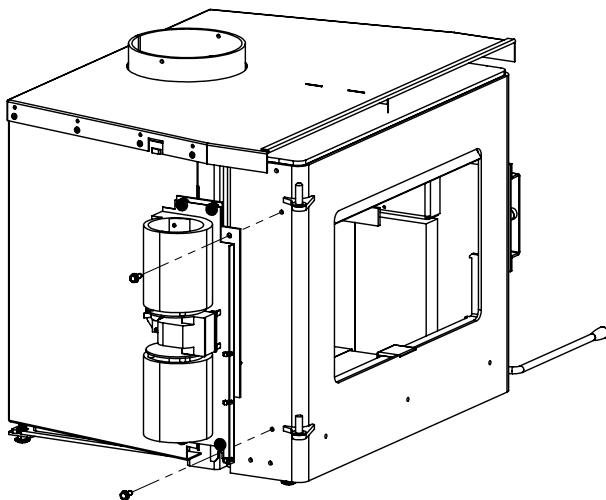
Figure 30: Fan Removal
