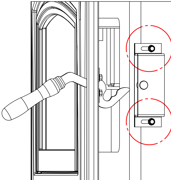
Figure 32: Latch Adjustment
