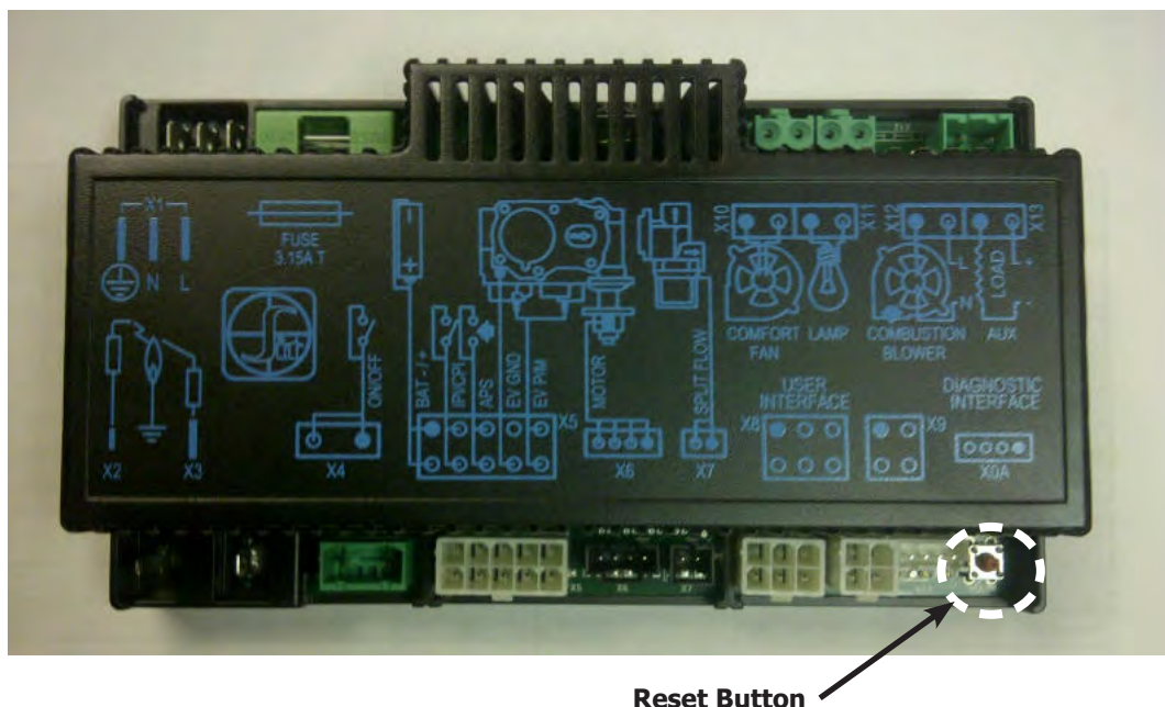
Figure 7: Integrated Fireplace Controller
