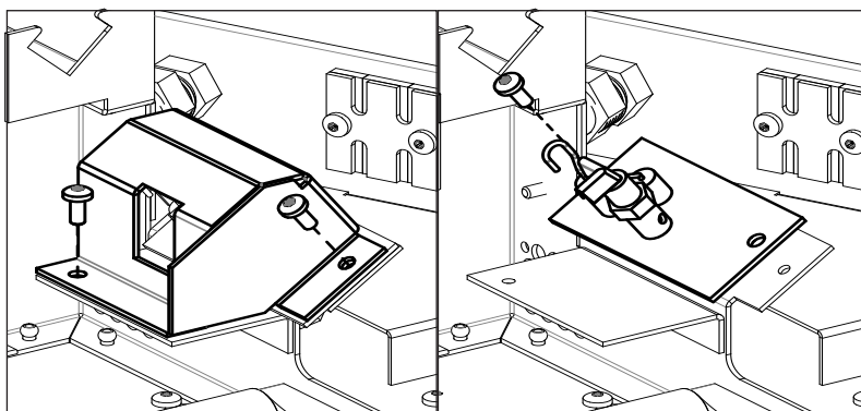
Figure 10: Pilot Shield & Pilot Removal
