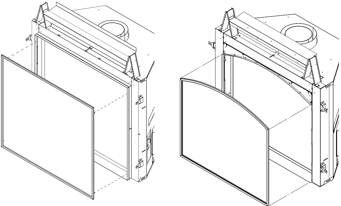
Figure 4: Safety Screen Removal (U37 and U37I-A models)
