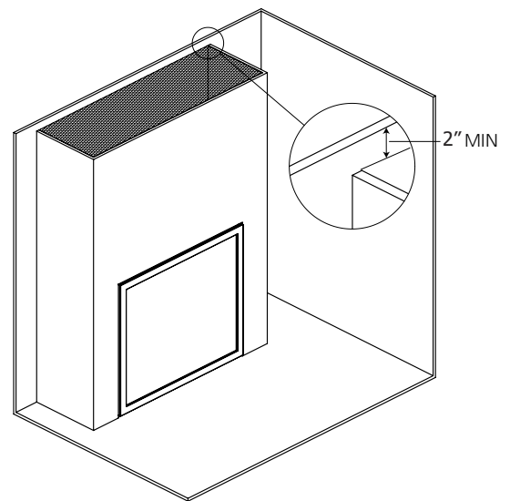
Figure 46: Open Chase Iso View
