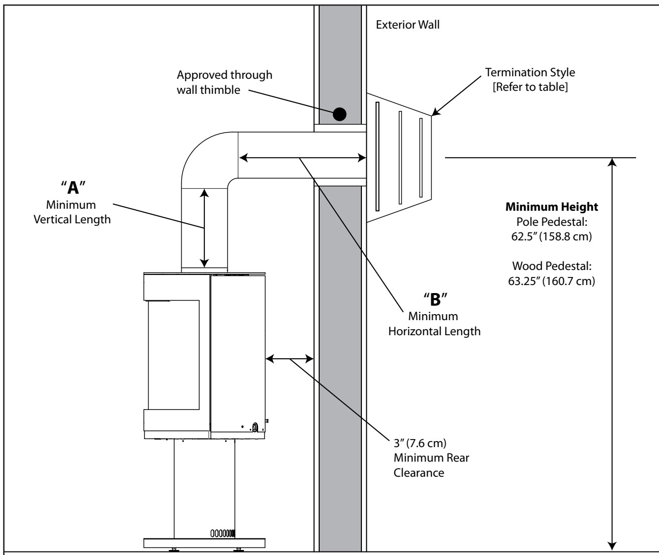
Figure 48: Minimum Vent Configuration - Top Vent
