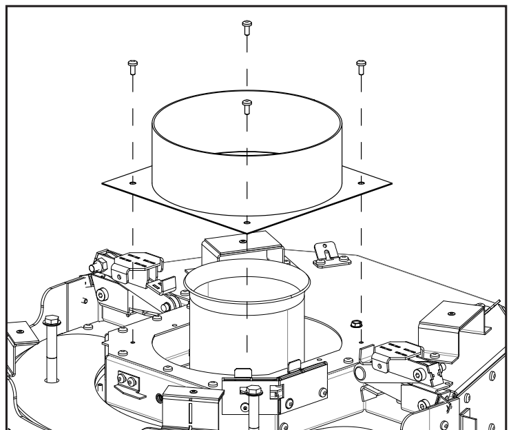
Figure 63: Vent Adapter Removal
