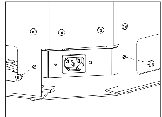
Figure 77: Electrical Plug Disconnect
