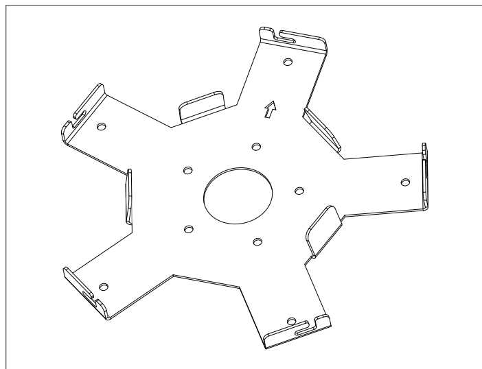
Figure 74: Pole Pedestal Anchor
