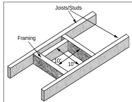
Figure 45: Vent Framing For Wall or Ceiling.
