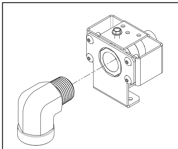
Figure 83: 1/2" Elbow Fitting Connection
