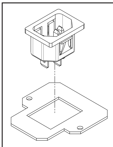
Figure 78: Electrical Adapter Plate
