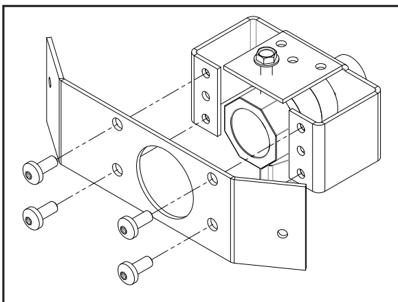
Figure 81: Gas Plate Removal
