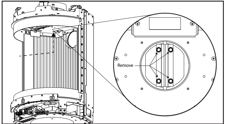
Figure 61: Restrictor Plate Removal
