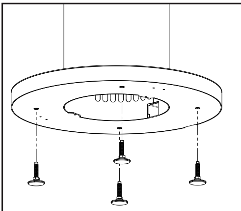
Figure 71: Pole Pedestal Leveling Feet
