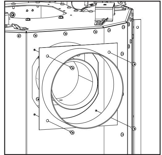
Figure 67: Vent Adapter Attachment
