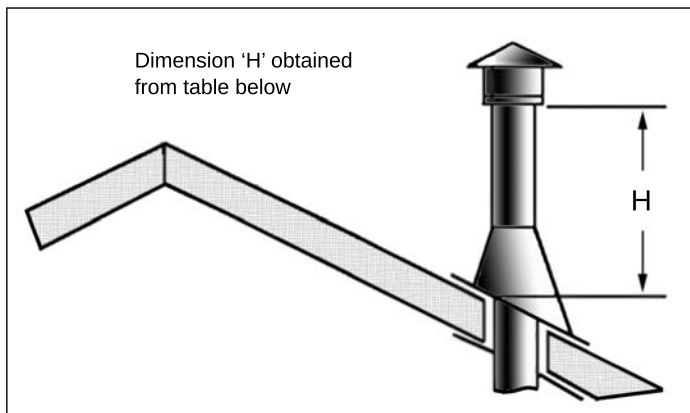
Figure 55: Height of Vertical Termination; Reference Table 8.
