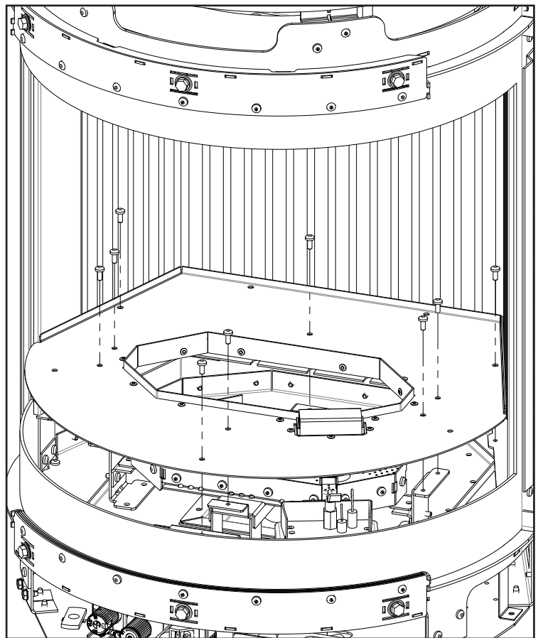
Figure 33: Burner Platform Removal
