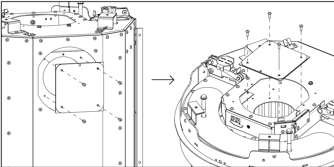
Figure 65: Inner Block-Off Plate Removal and Attachment
