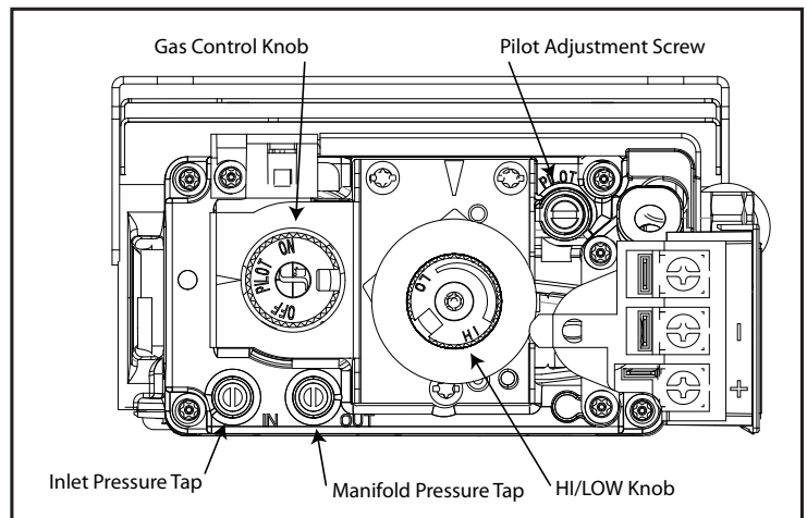
Figure 58: Fully Labeled Gas Valve
