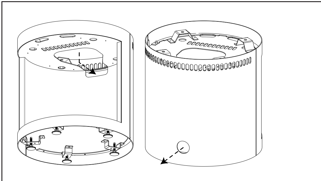
Figure 86: Wood Pedestal Gas & Electrical Rerouting
