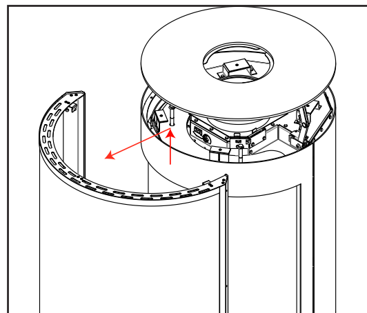
Figure 13: Safety Screen Removal
