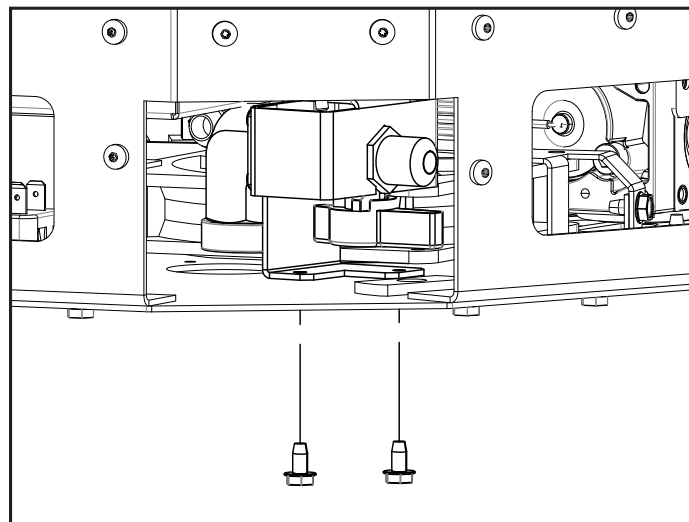
Figure 84: Gas Connection Re-installation
