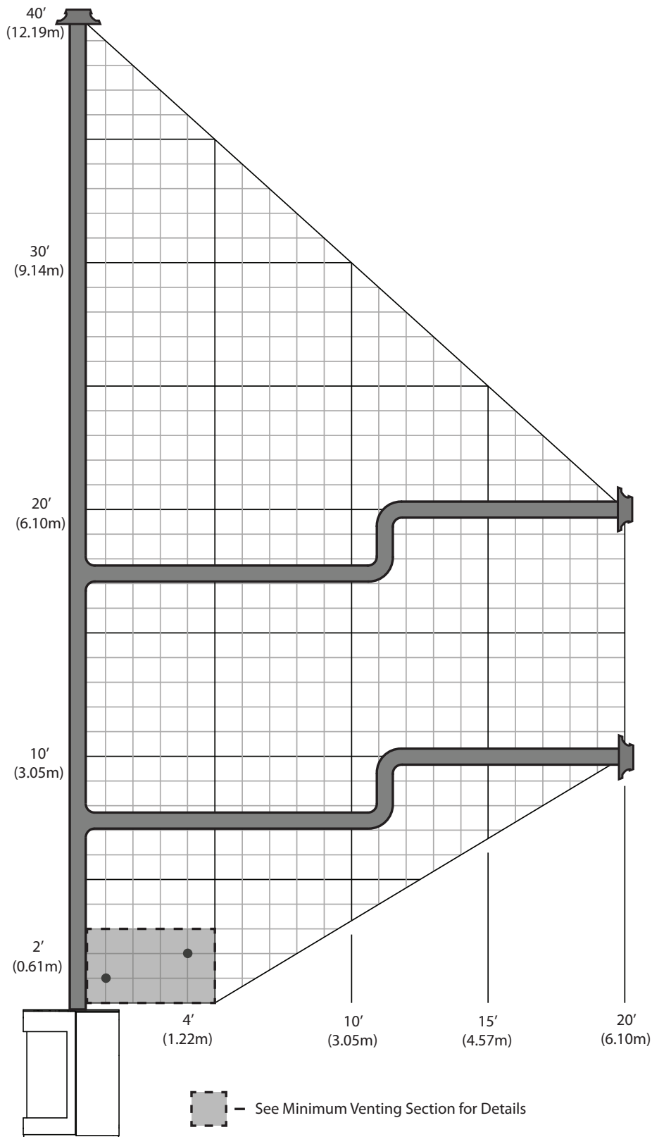
Figure 49: Top Vent Configuration Diagram - NG
