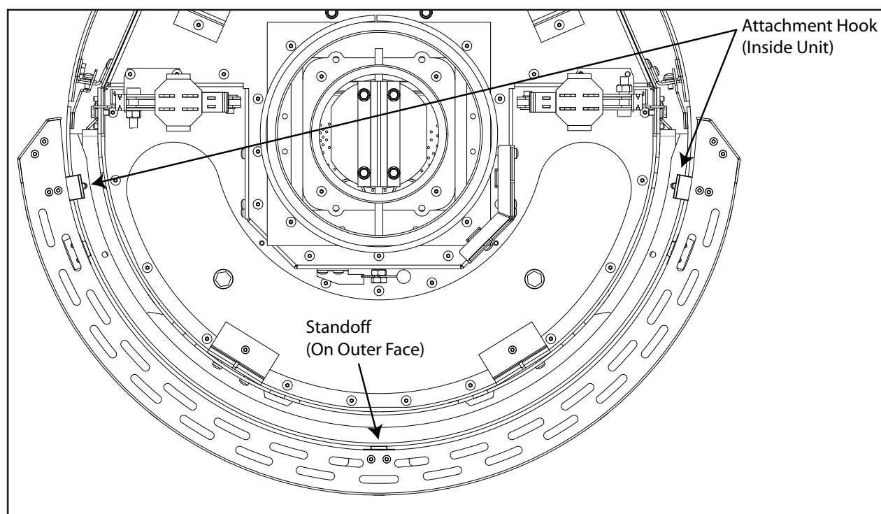
Figure 14: Safety Screen Attachment (Top-Down View)
