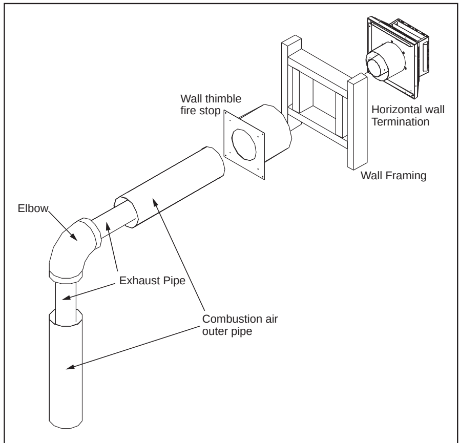
Figure 53: Horizontal Vent Termination
