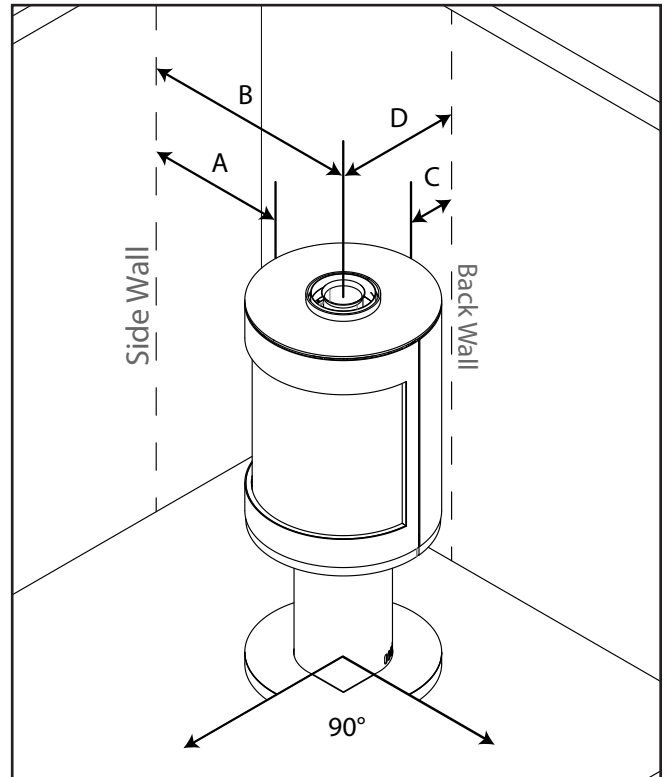
Figure 42: Clearance to Combustibles
