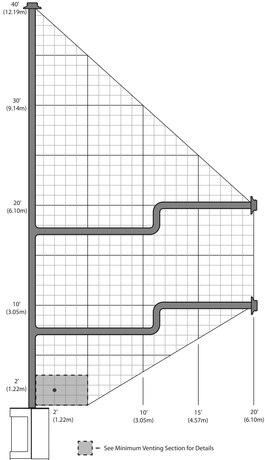
Figure 50: Top Vent Configuration Diagram - LP
