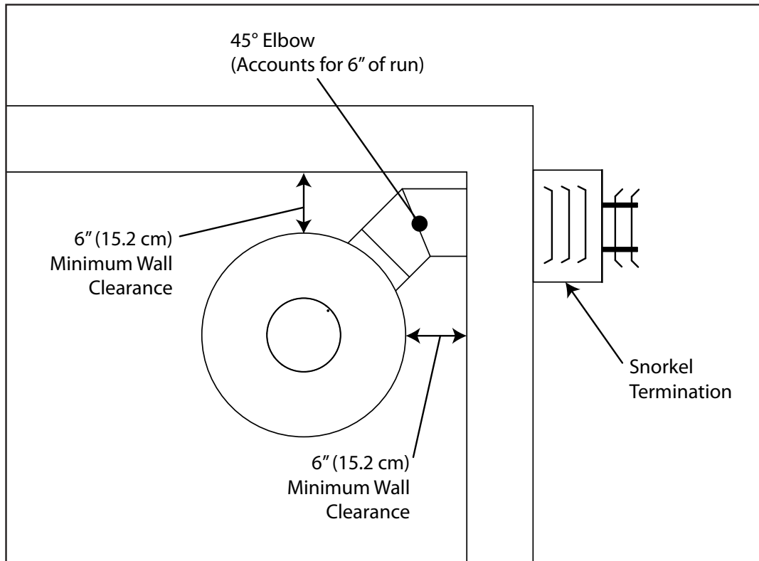
Figure 52: Rear Vent Corner Install Venting - Top View
