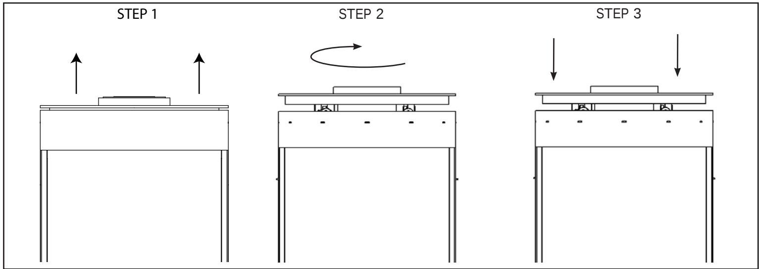
Figure 10: Lifting the Top Plate
