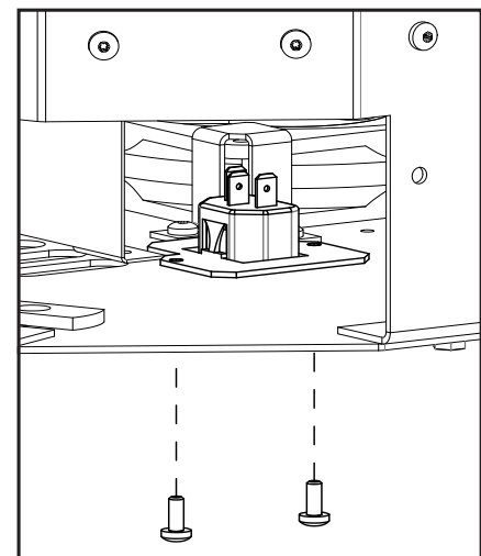
Figure 79: Electrical Plug Connection
