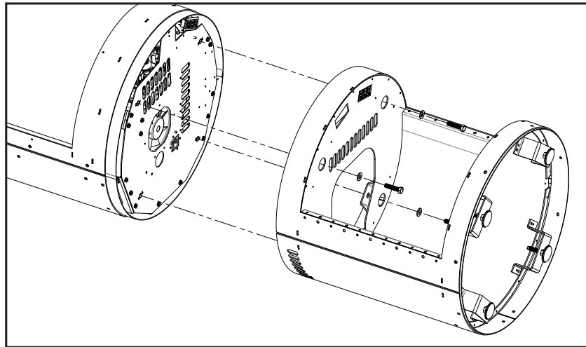
Figure 73: Wood Pedestal Installation v
