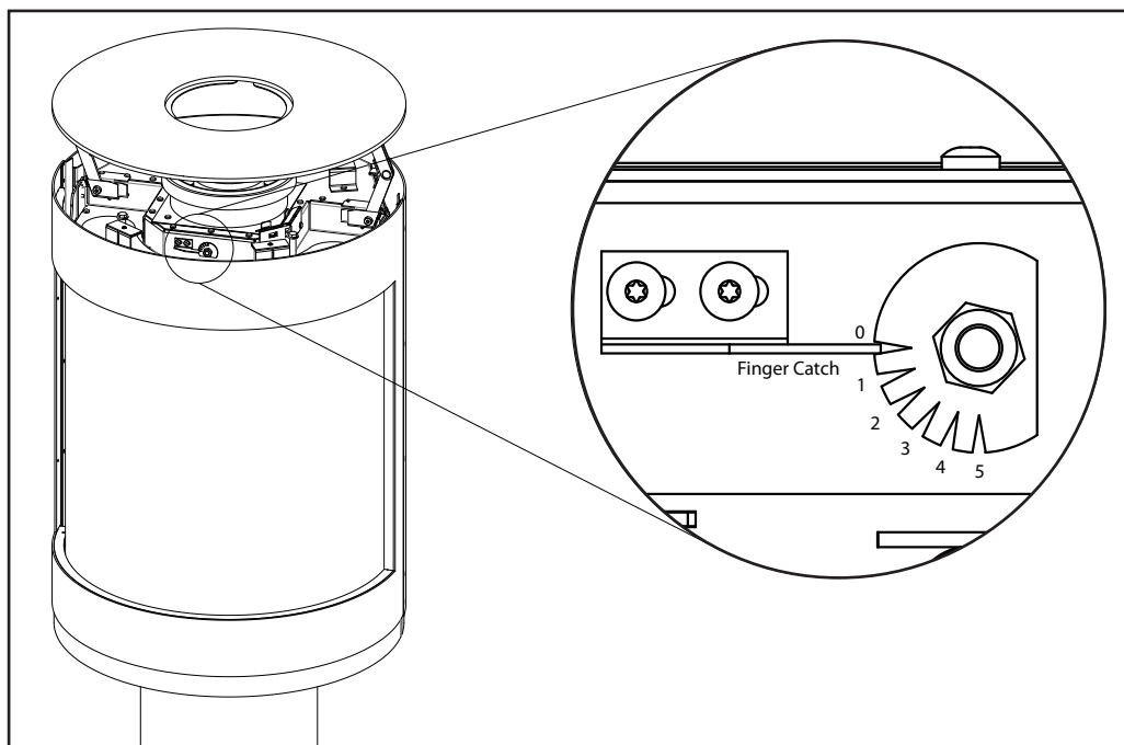
Figure 47: Exhaust Restrictor
