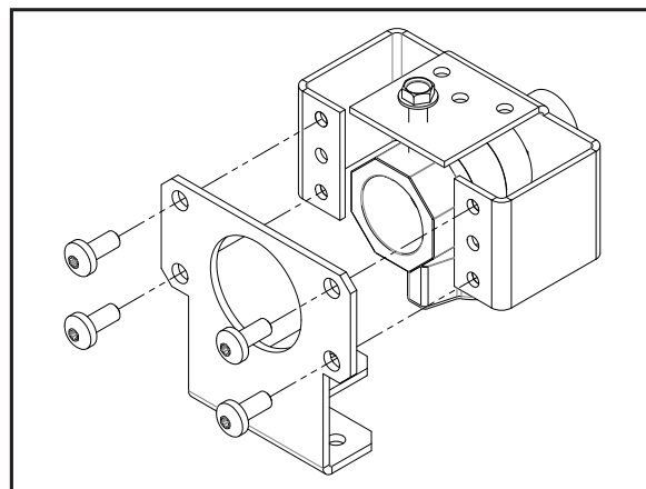
Figure 82: Gas Adapter Connection
