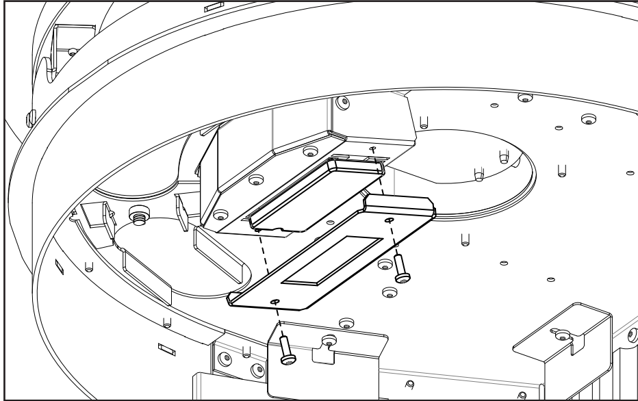
Figure 24: Top Light Removal
