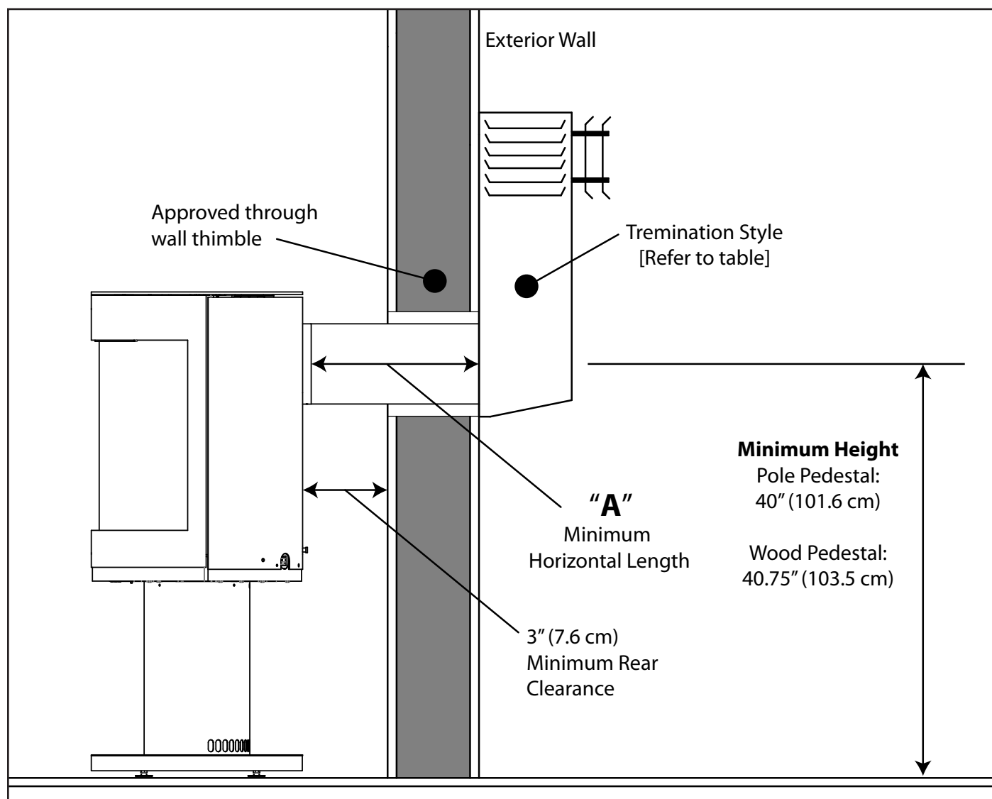
Figure 51: Minimum Vent Configuration - Rear Vent
