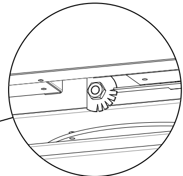
Figure 59: Restrictor Setting 1
