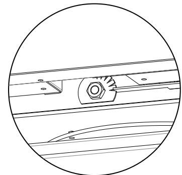
Figure 60: Restrictor Setting 6
