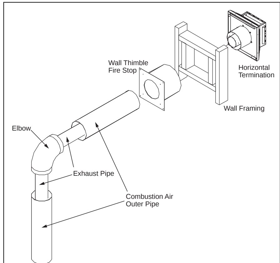
Figure 61: Horizontal Vent Termination
