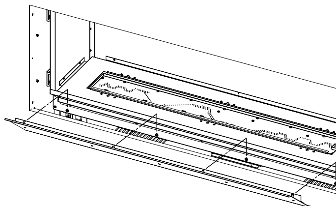
Figure 22: Removing Intake Shield
