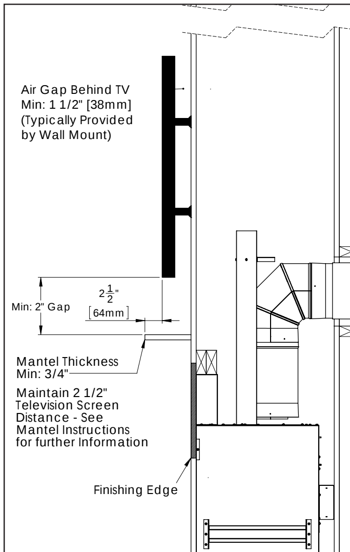
Figure 42 Minimum TV Install Clearances
