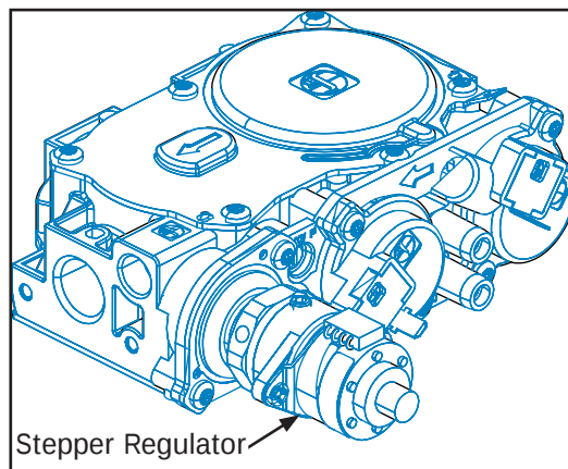
Figure 11: 885 Gas Valve
