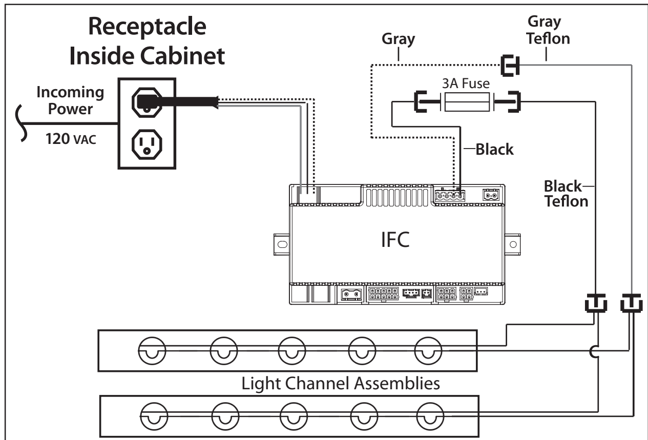
Figure 59 Light Kit Wiring Diagram. C60I Light Kit Wiring Diagram
