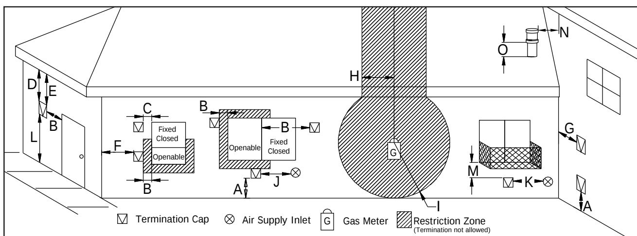
Figure 44 Vent Termination Restrictions, refer to Table 3
