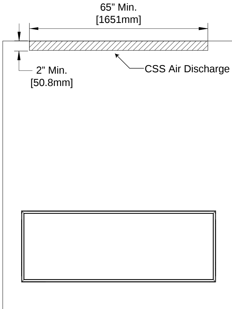
Figure 24 CSS Outlet
