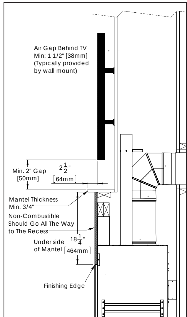
Figure 43 Recess Minimum TV Install Clearances
