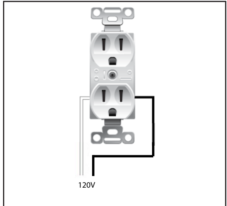
Figure 57 C60 Wiring Diagram
