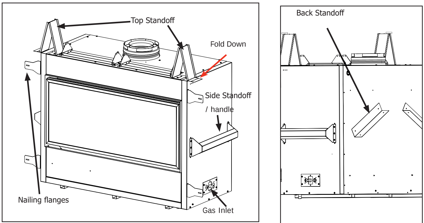
Figure 13: Fireplace Install Preperation
