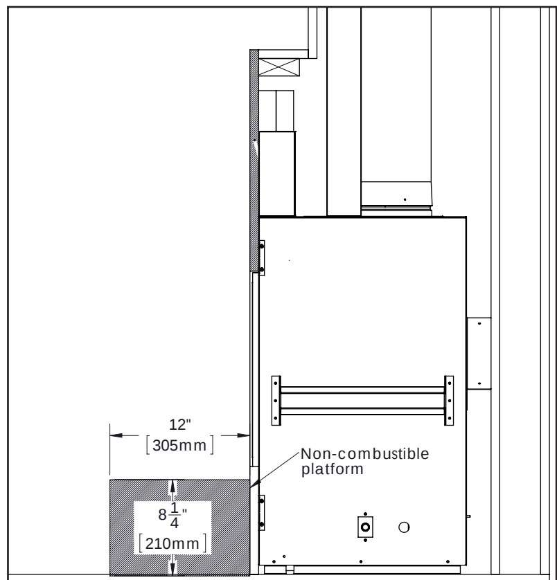
Figure 35: Non-Combustible Platform
