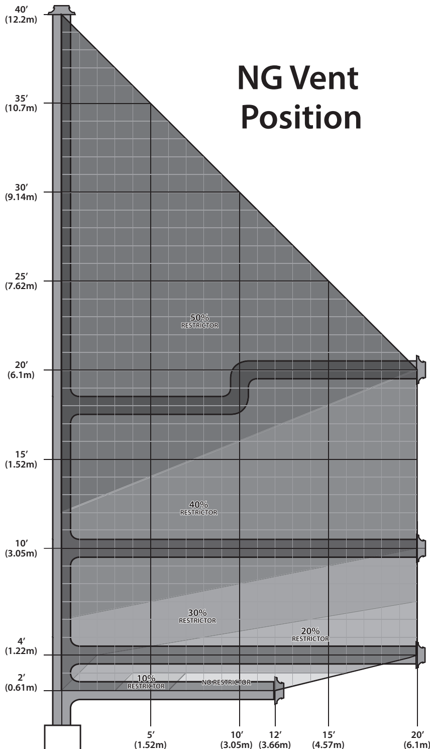
Figure 46 Natural Gas Vent Graph
