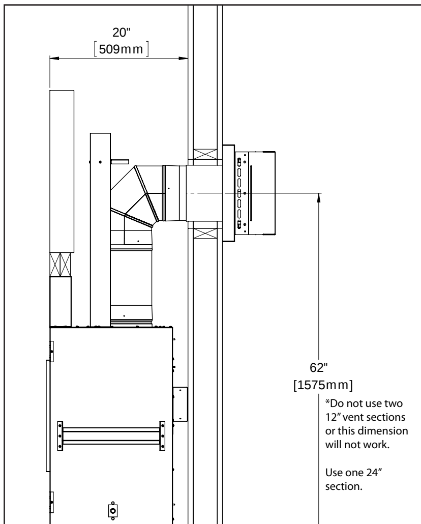
Figure 34: Minimum Horizontal Framing
