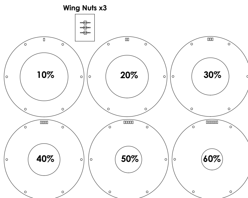
Figure 49 RestrictorRing Kit
