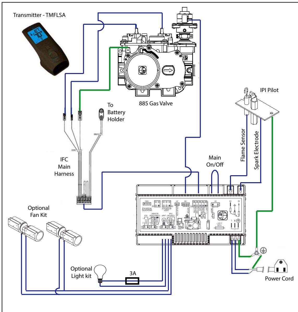
Figure 56 C60 Wiring Diagram
