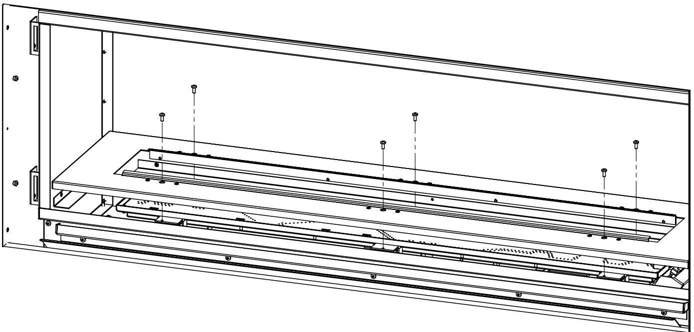
Figure 60 Standard Burner Tray Install/Removal
