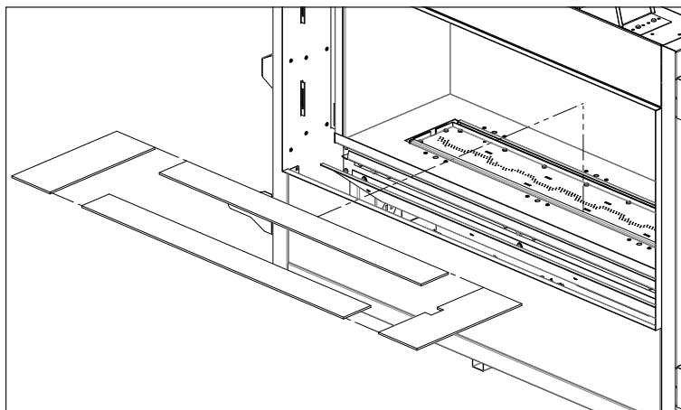
Figure 61 Burner Bezel Placement
