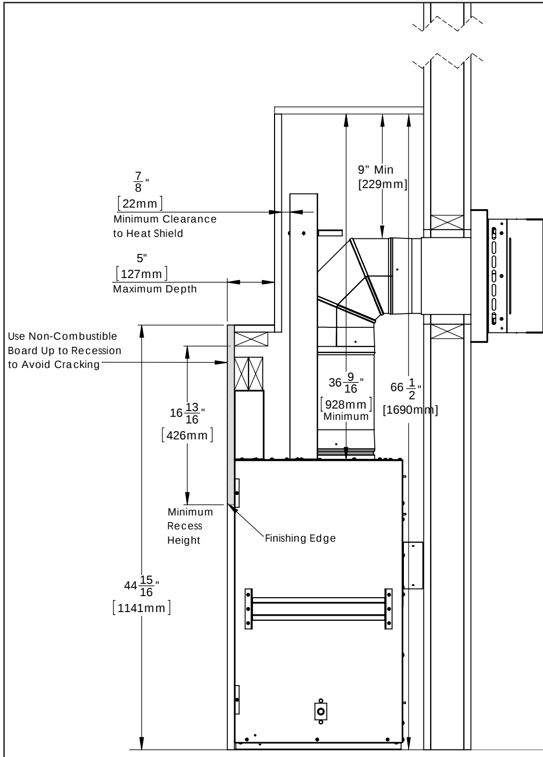
Figure 37: Install Dimensions with Recess
