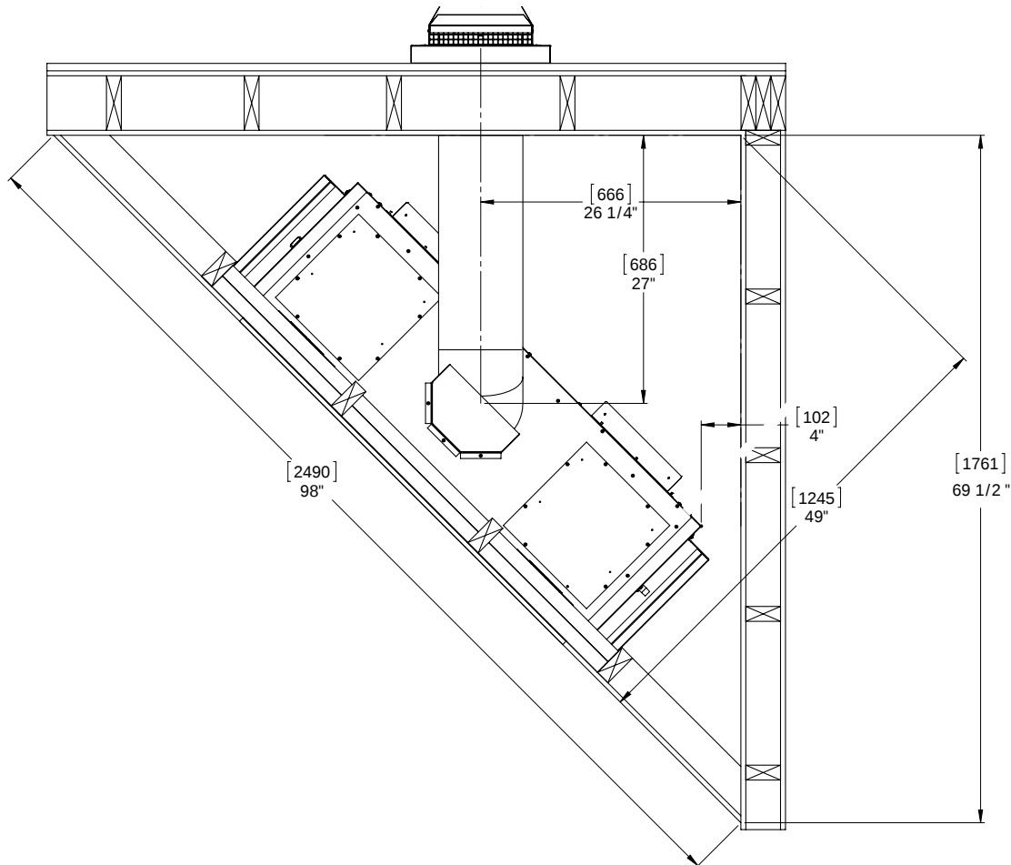
Figure 38. Dimensions for a Corner Installation
