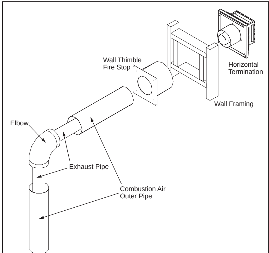
Figure 49. Horizontal Vent Termination
