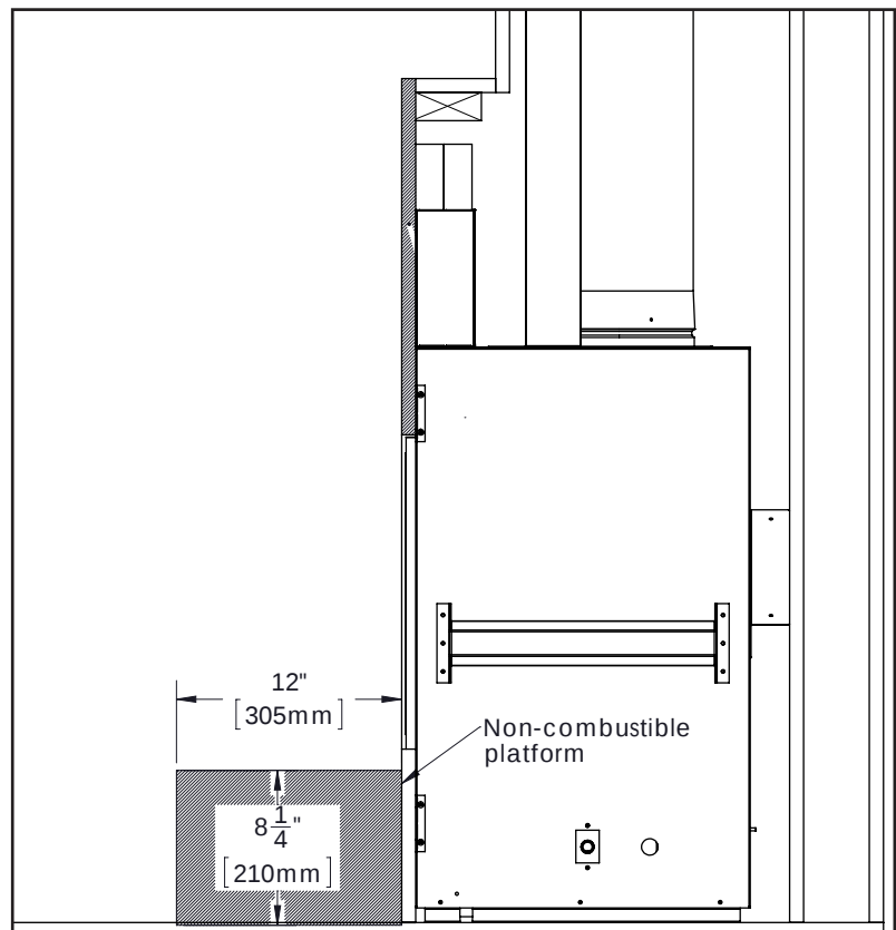
Figure 35: Non-Combustible Platform
