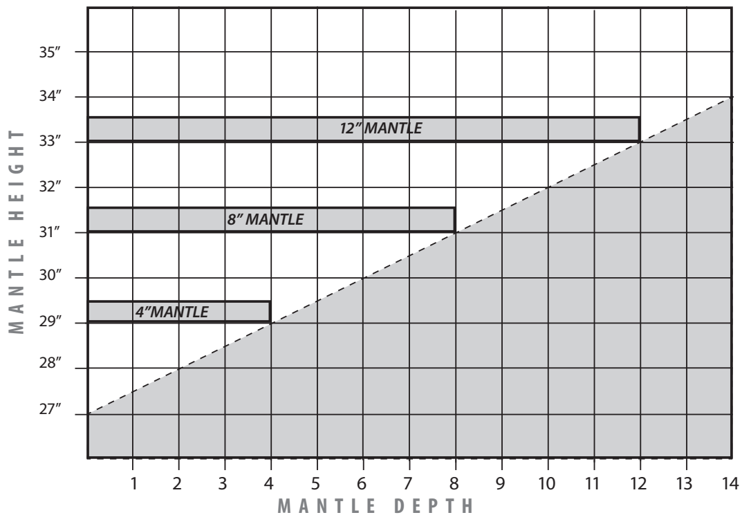
Figure 36(b): Minimum Mantel Height -- CSS Activated
