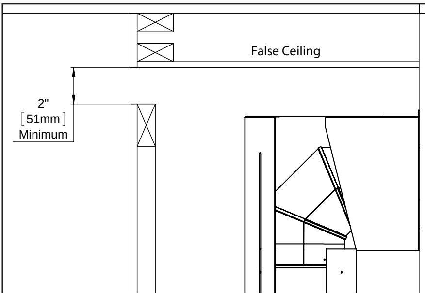
Figure 26: False Ceiling
