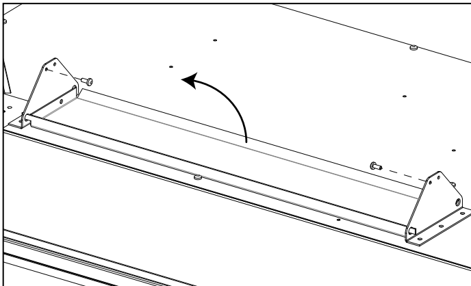
Figure 22 CSS flaps - closed
