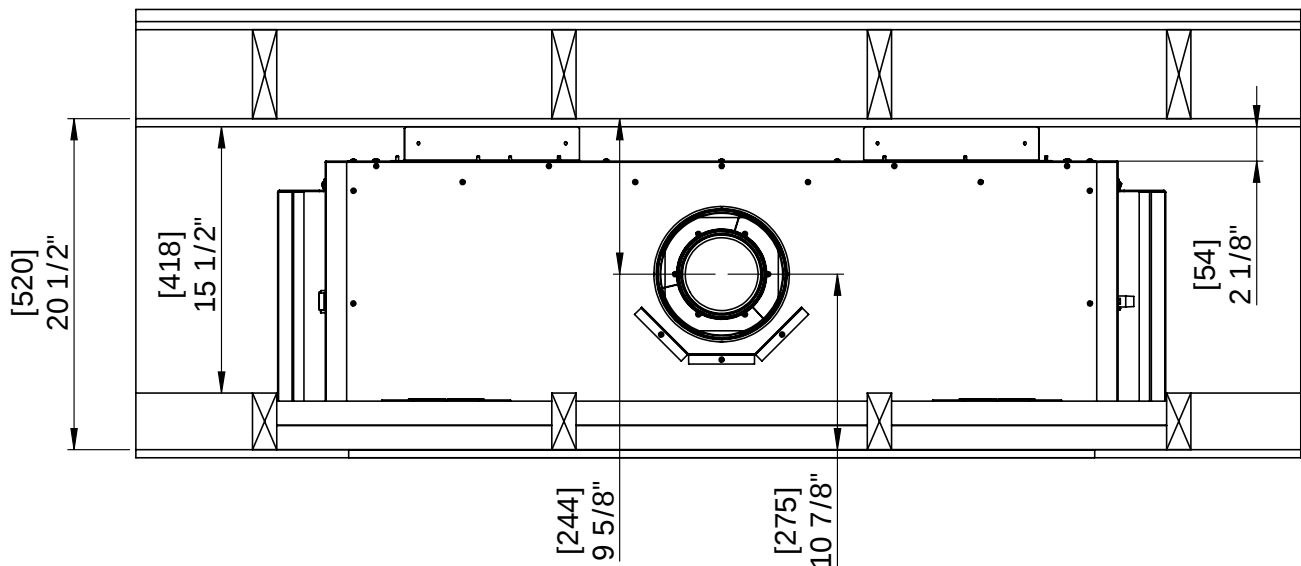
Figure 40(b). Dimensions for a Vertical Installation
