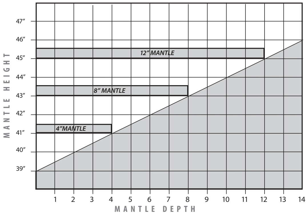
Figure 36(a): Minimum Mantel Height
