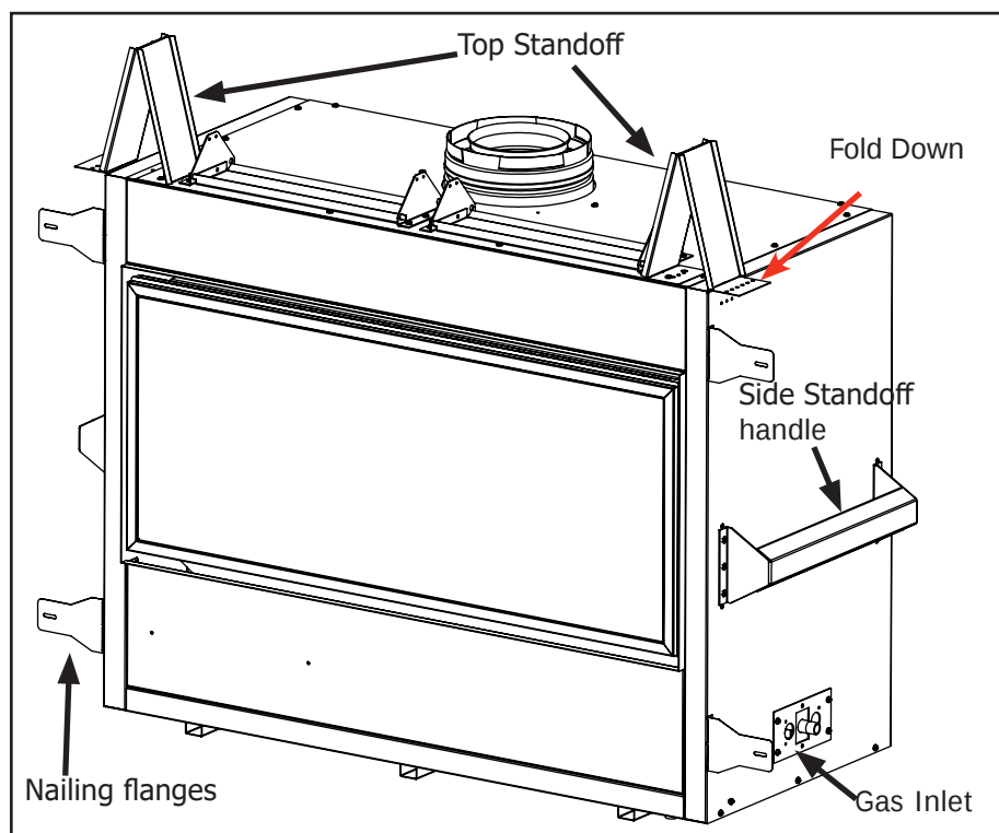
Figure 13: Fireplace Install Prep
