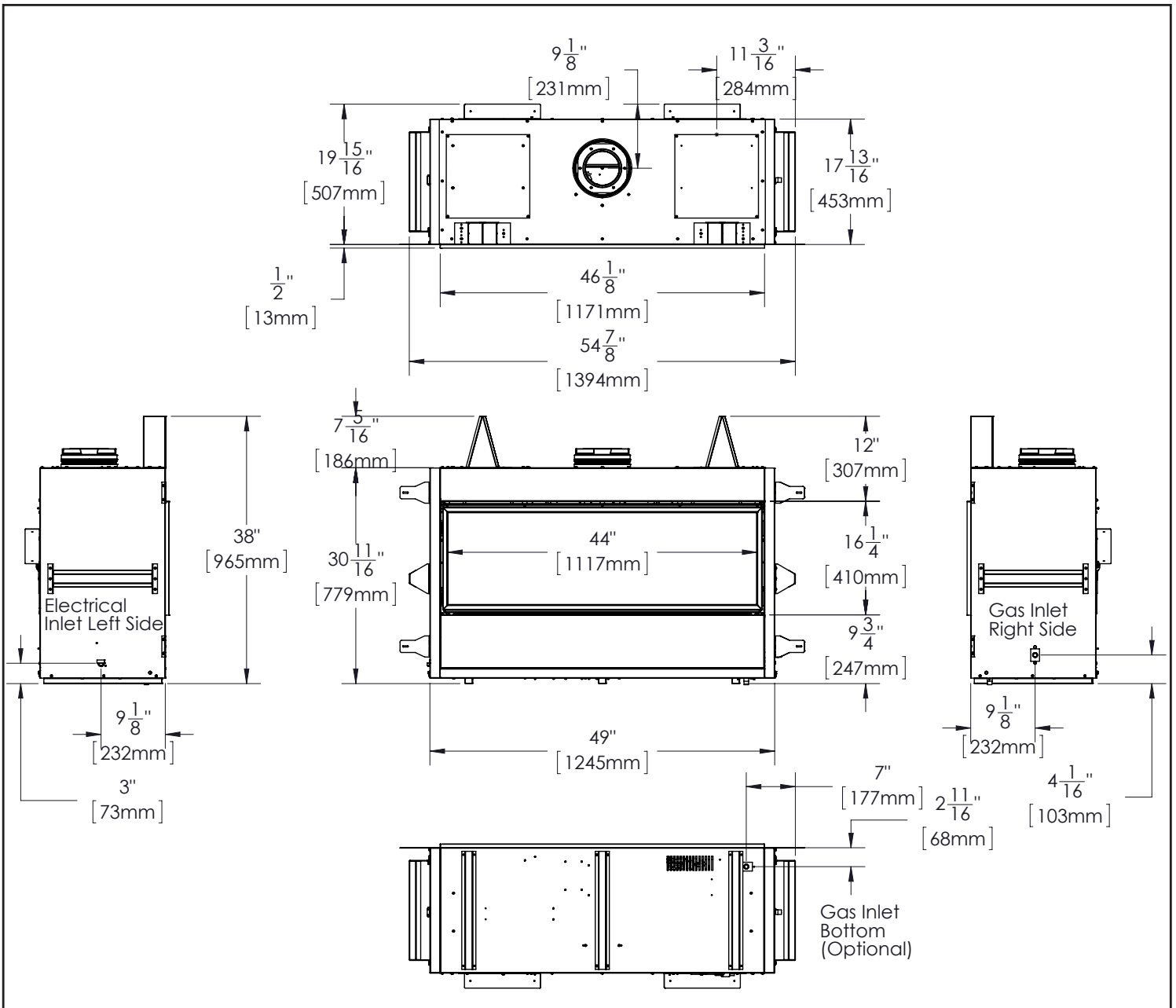
Figure 1: Unit Dimensions
