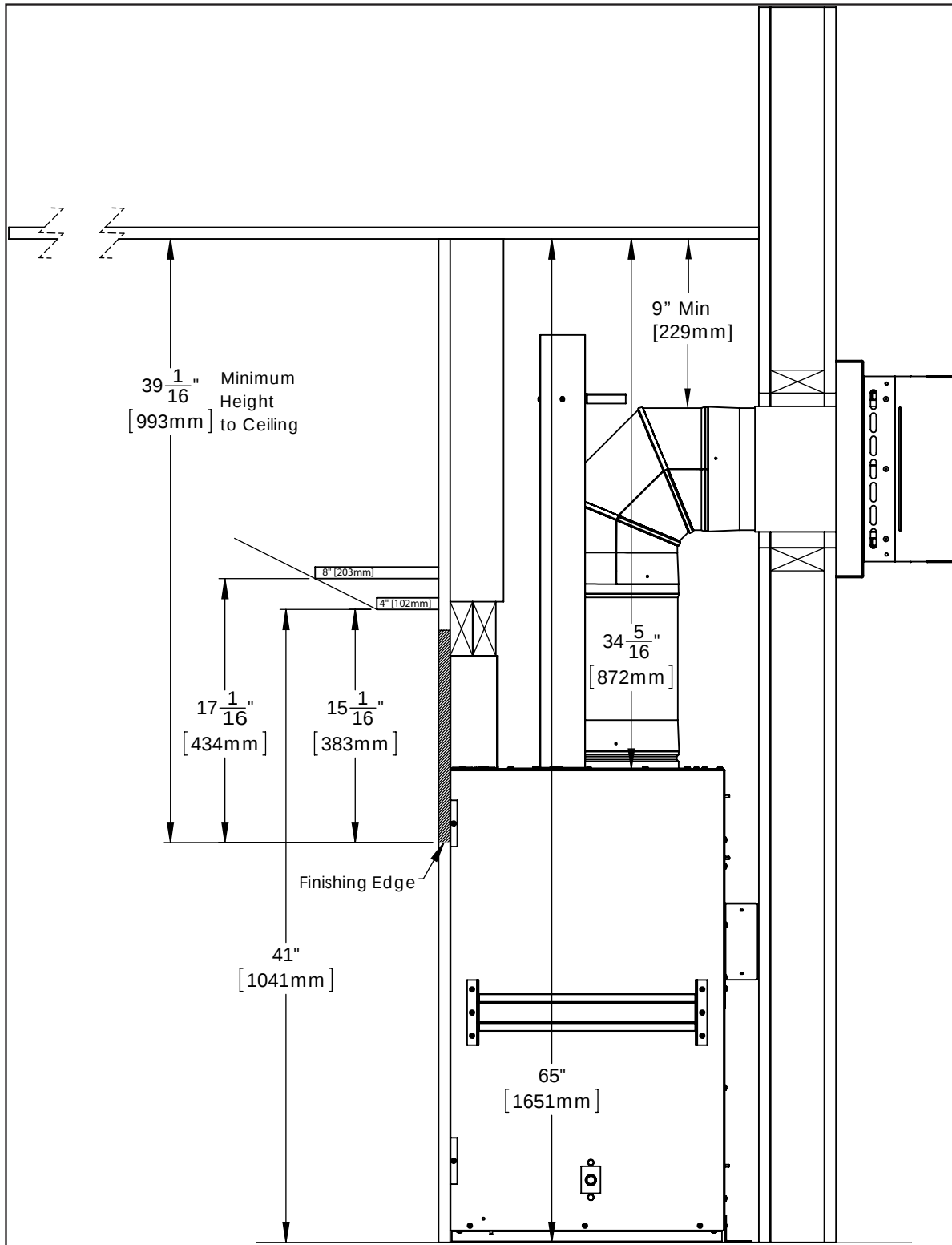
Figure 36(c): Install Dimensions with Mantel
