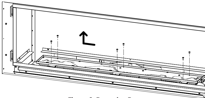
Figure 6: Removing Burner
