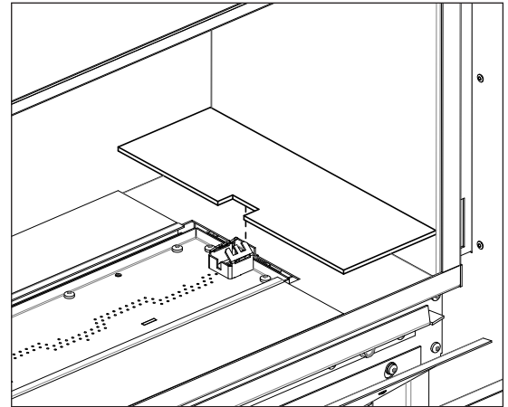
Figure 60: Bezel Placement Around Pilot
