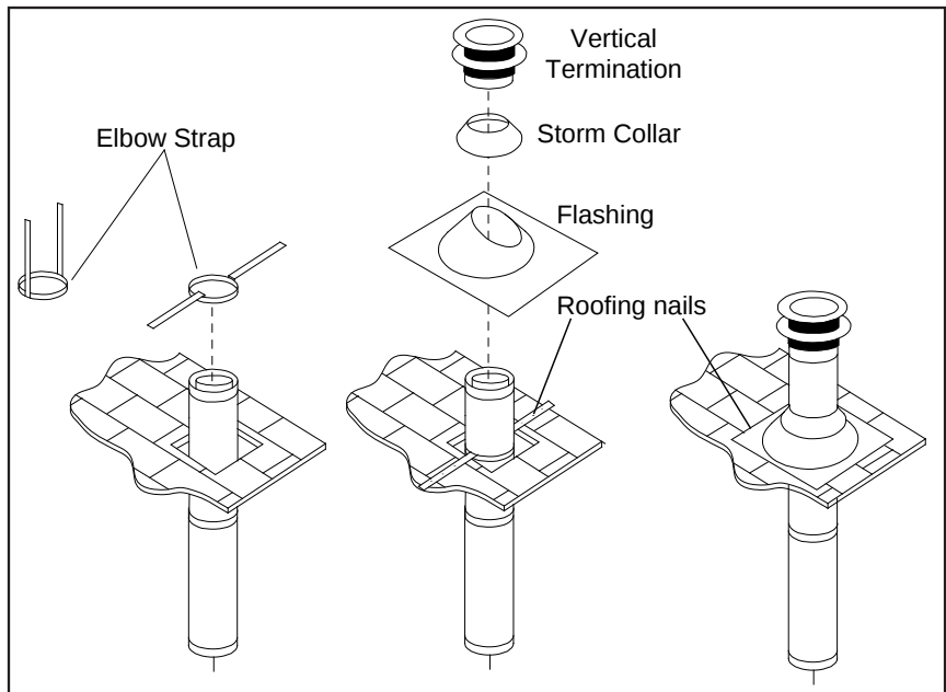
Figure 50(a). Vertical Vent Termination
