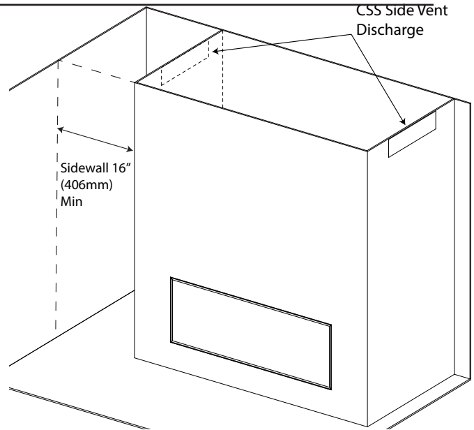
Figure 25 CSS Side Vent
