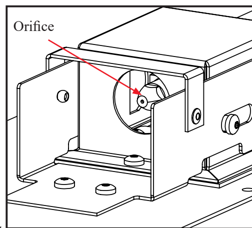
Figure 10: Orifice location
