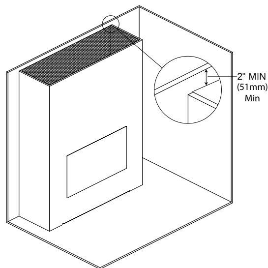
Figure 29: Open Chase Iso View
