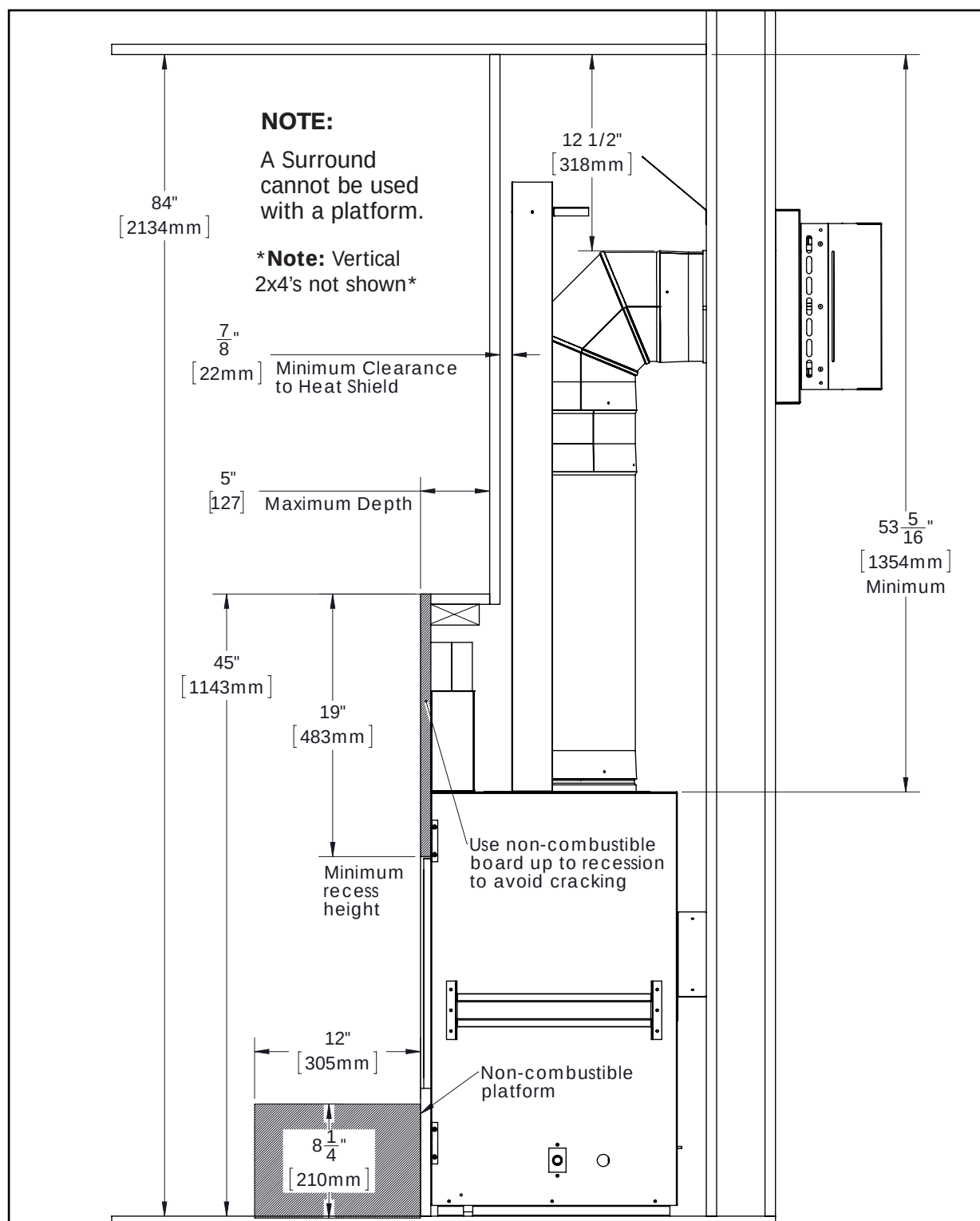
Figure 38: Install Dimensions with Platform
