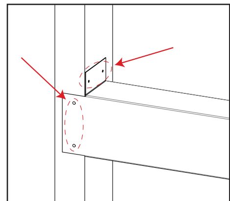
Figure 17: Steel Stud Installation
