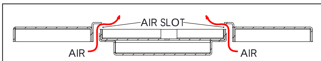
Figure 63: Burner Side Cross Section
