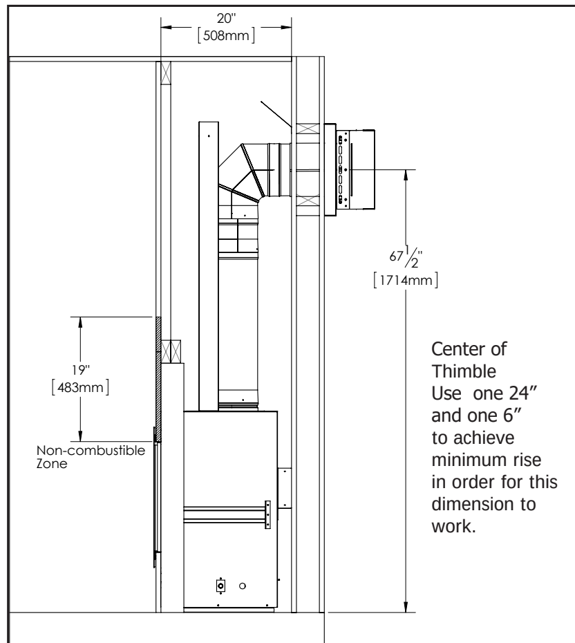
Figure 34: Minimum Horizontal Venting
