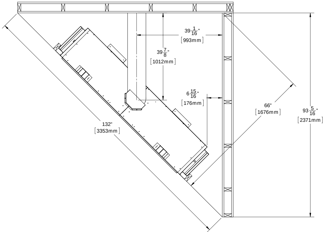
Figure 39. Dimensions for a Corner Installation
