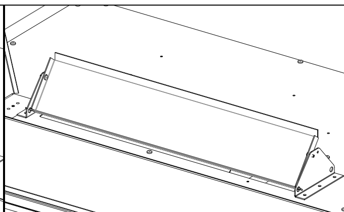
Figure 23 CSS flaps - open
