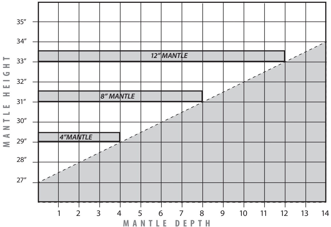
Figure 35(b): Minimum Mantel Height with CSS
