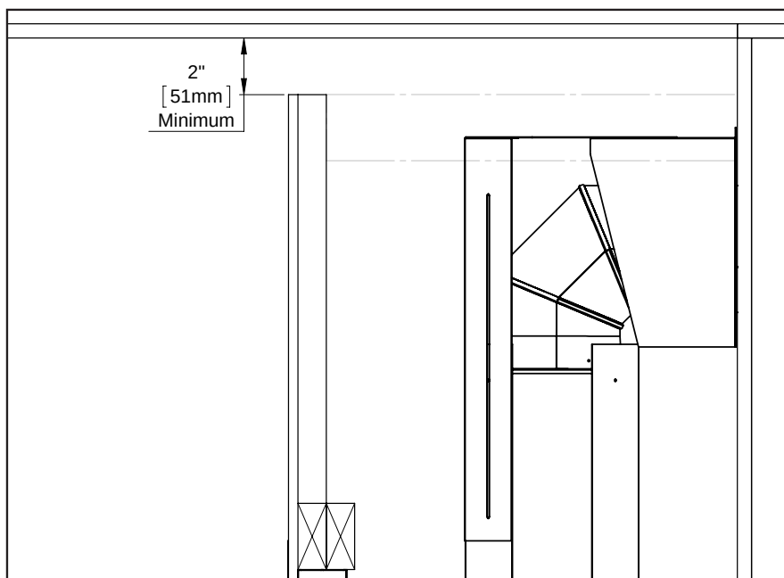
Figure 28: Open Chase
