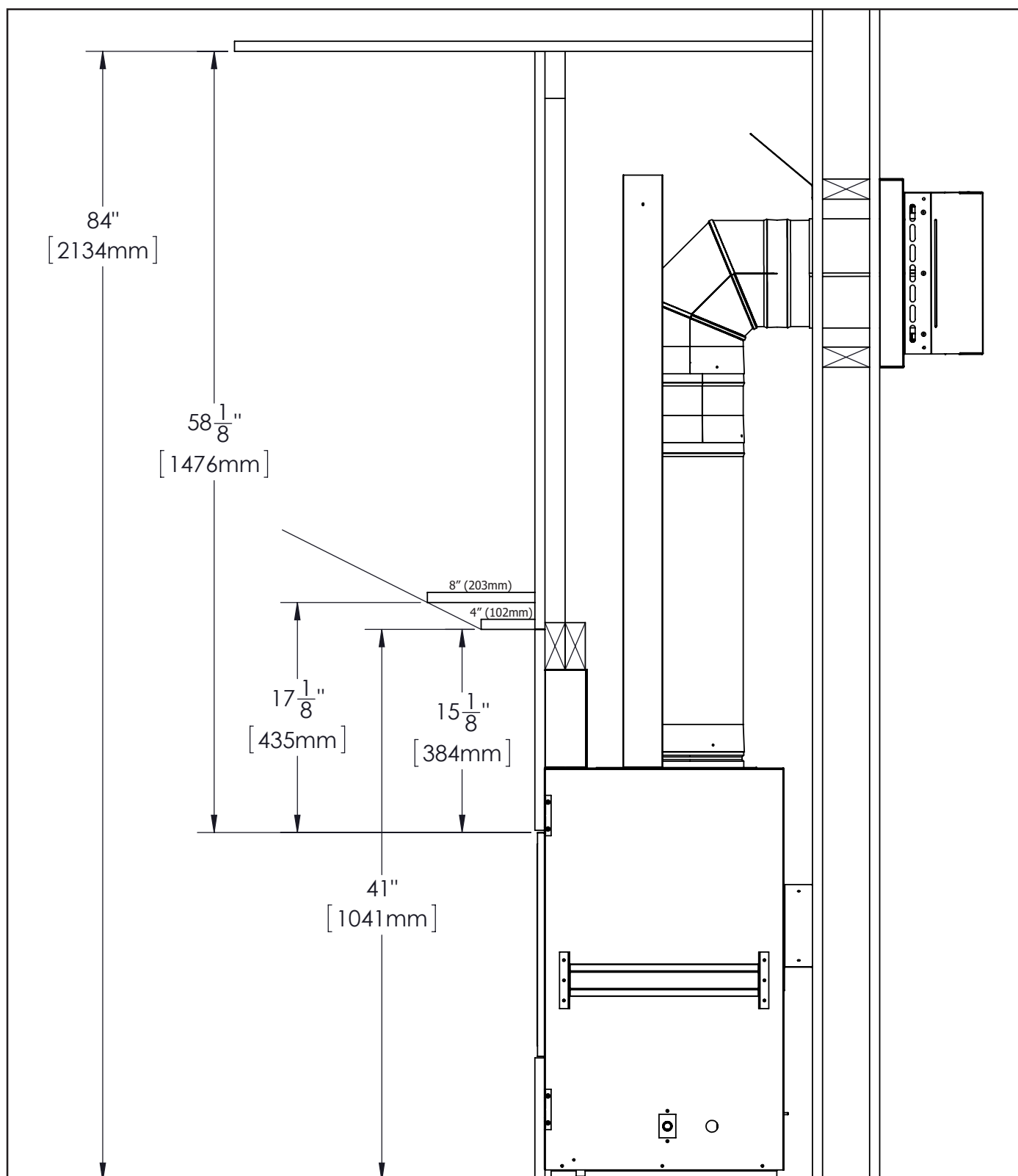
Figure 36: Install Dimensions with Mantel
