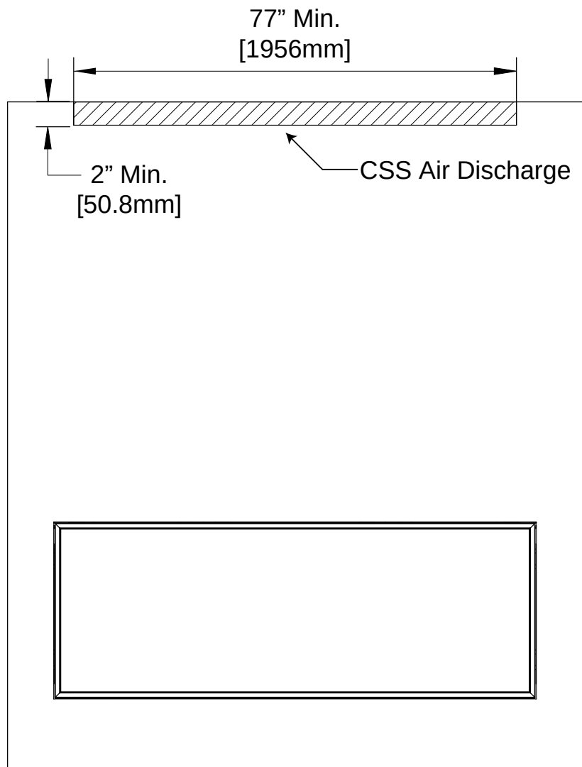
Figure 24 CSS Outlet
