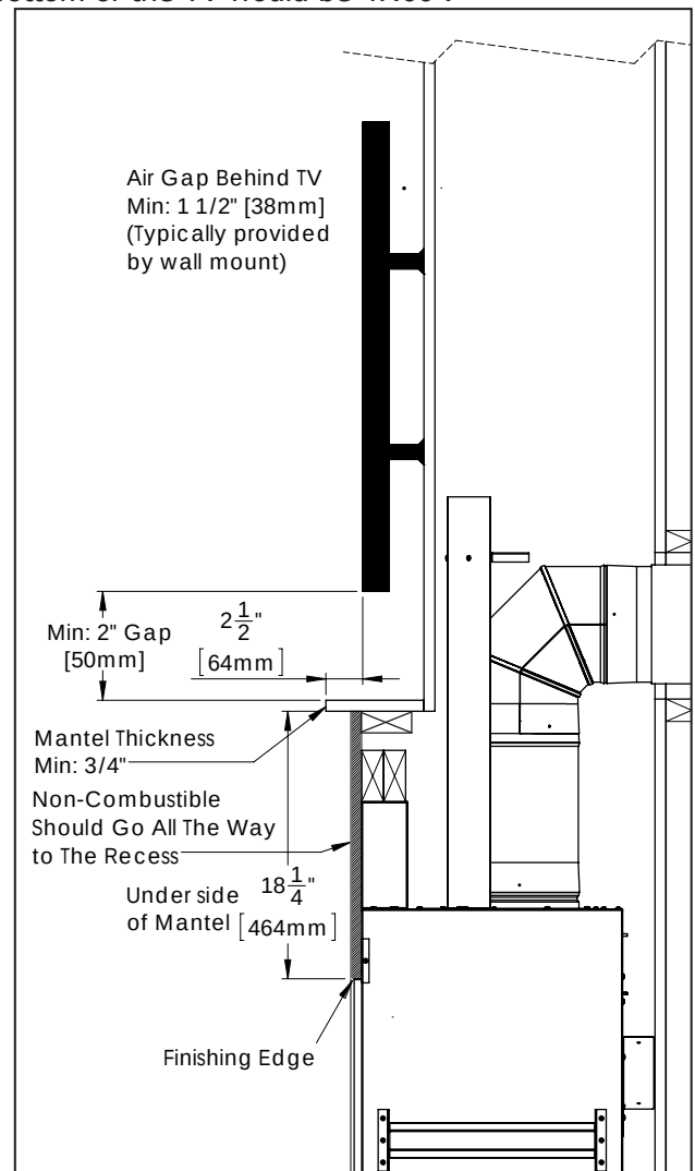
Figure 44. Recess Minimum TV Install Clearances
