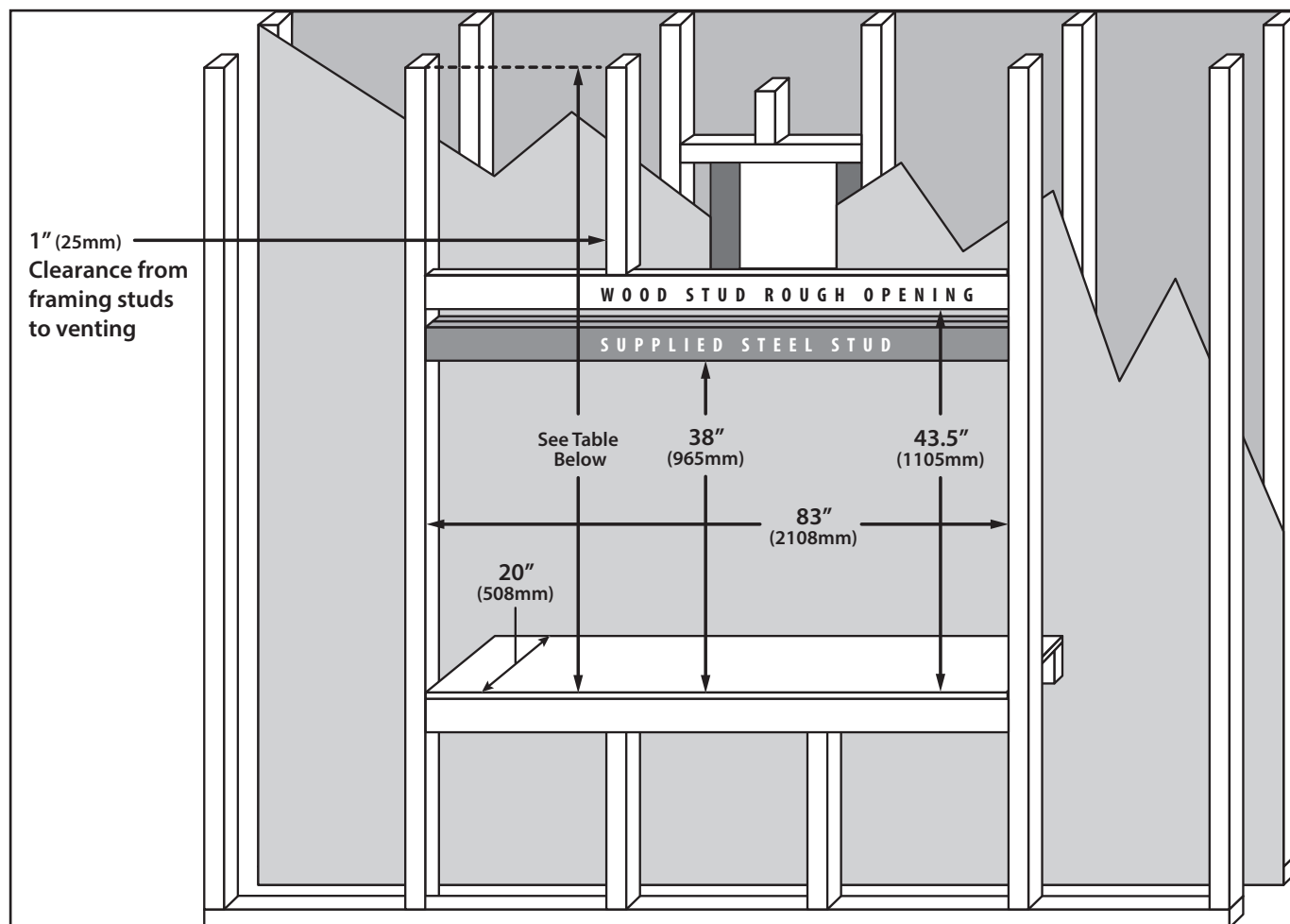
Figure 18. Construction Framing Dimensions
