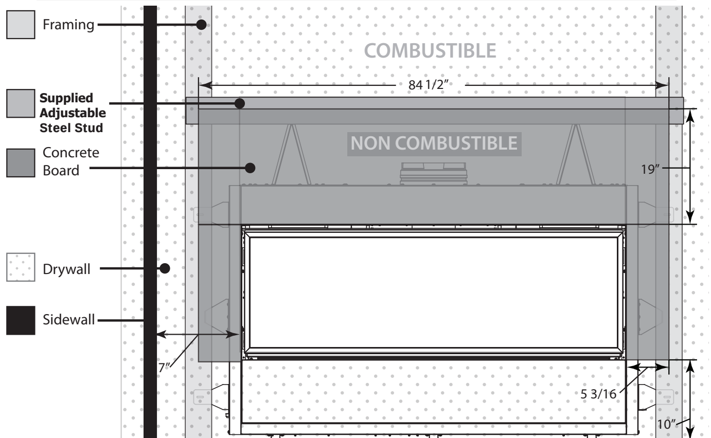
Figure 19 Finishing Non-Combustible Zone
