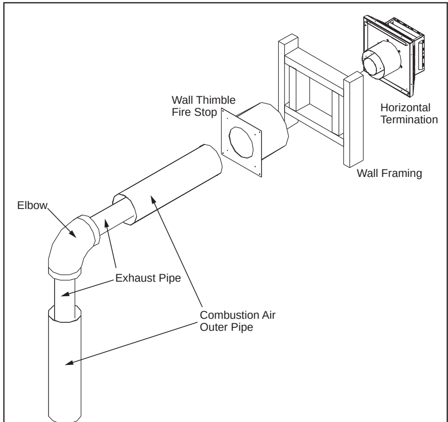
Figure 50. Horizontal Vent Termination
