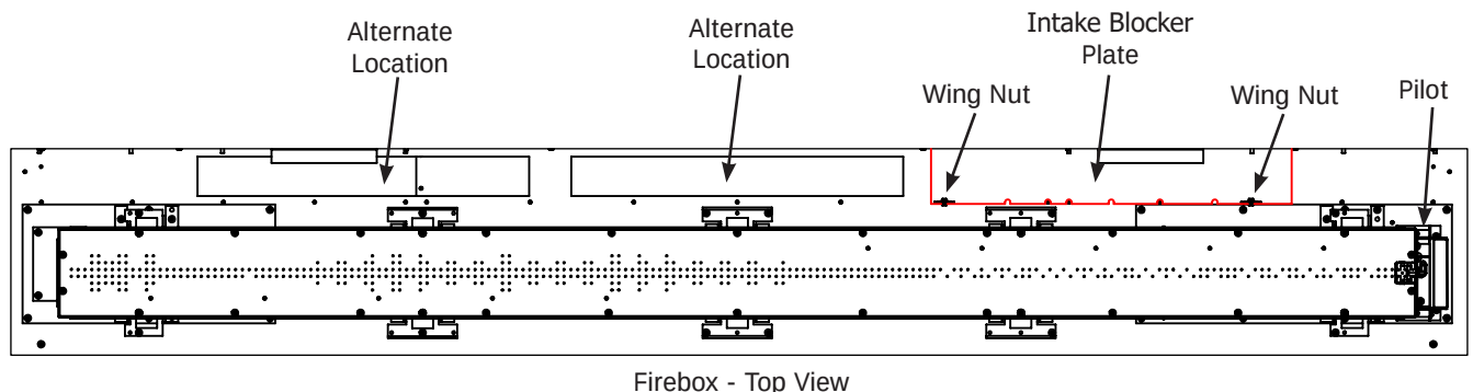
Figure 49. Intake Blocker Plate
