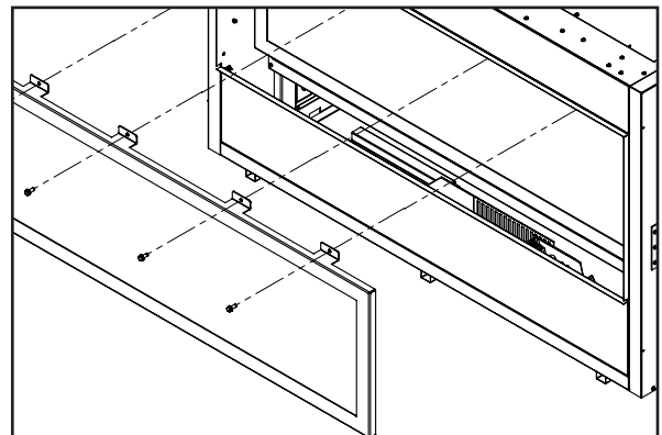
Figure 5(b). Door Removal Motion
