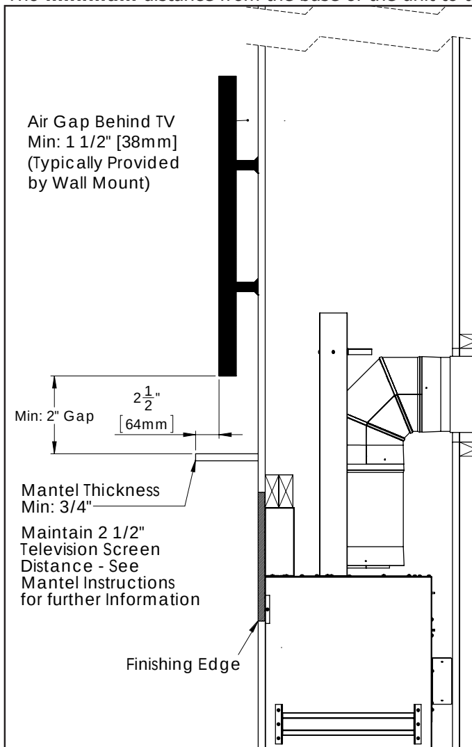
Figure 43. Minimum TV Install Clearances
