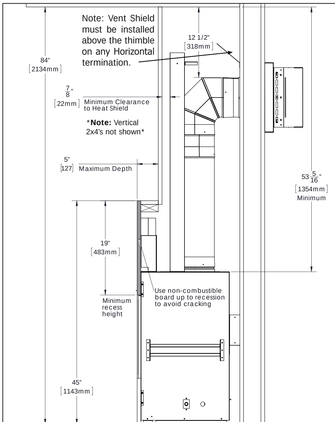
Figure 37: Install Dimensions with Recess
