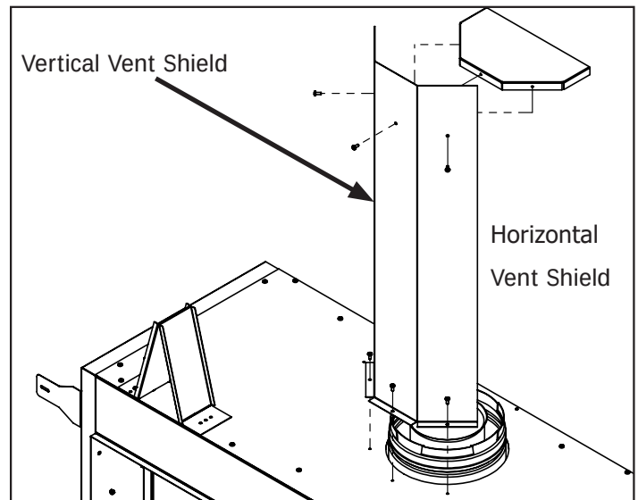
Figure 40. Vent Shielding Install
