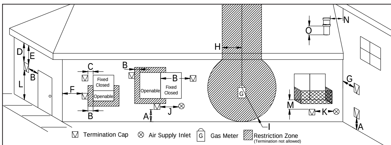
Figure 45. Vent Termination Restrictions, refer to Table 3
