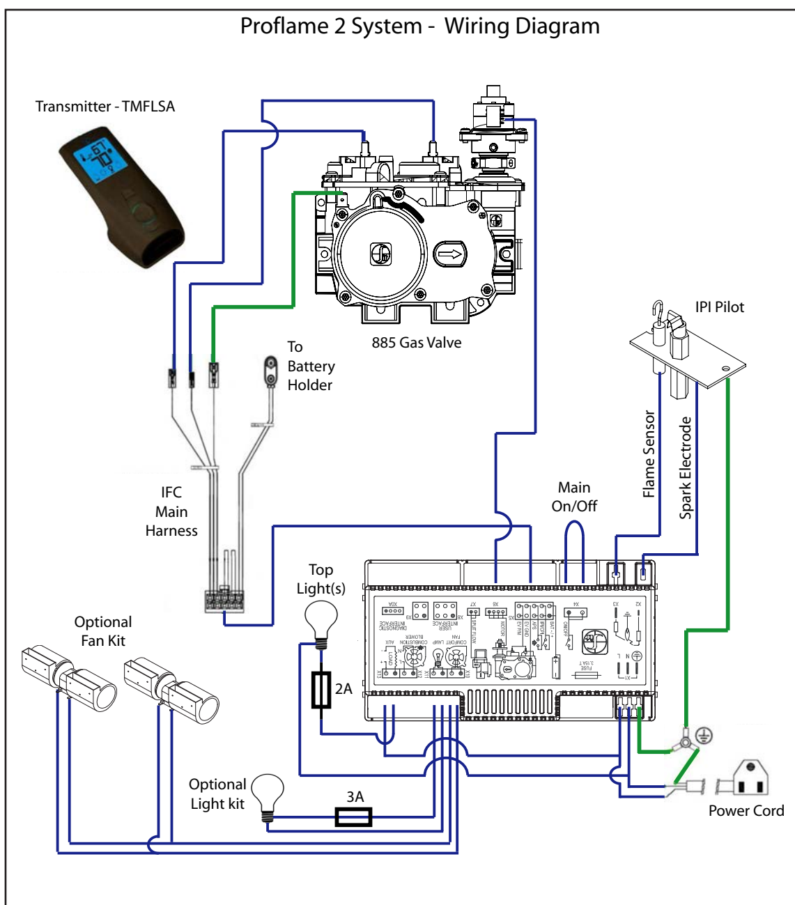
Figure 56: C72I Wiring Diagram
