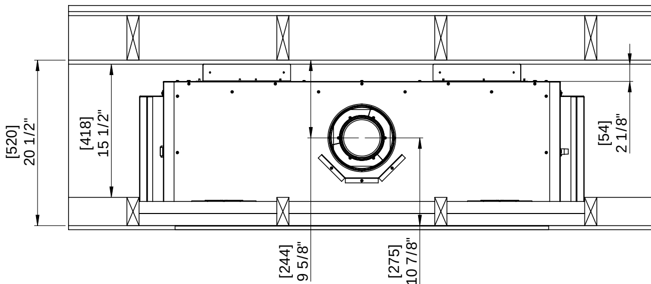
Figure 42. Dimensions for a Vertical Installation
