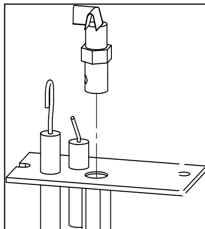
Figure 9. Pilot Orifice
