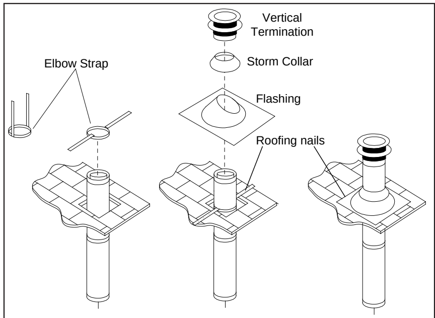
Figure 51. Vertical Vent Termination
