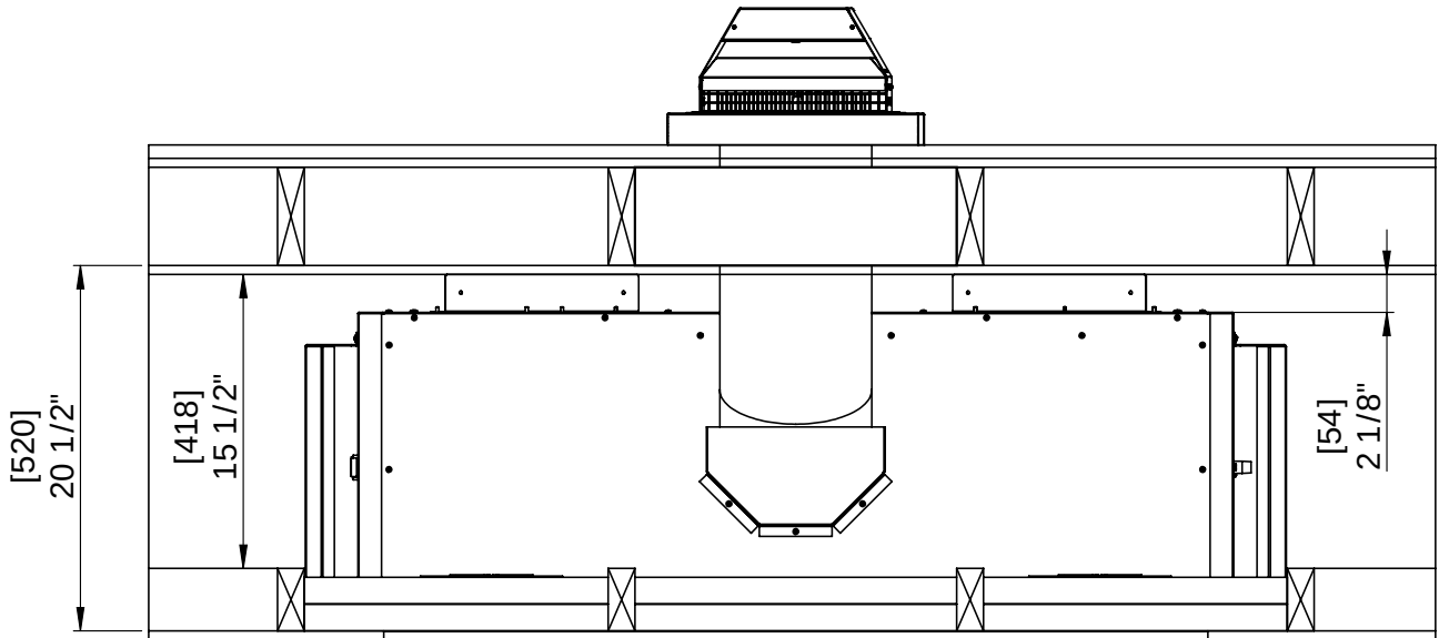
Figure 41. Dimensions for a Horizontal Installation
