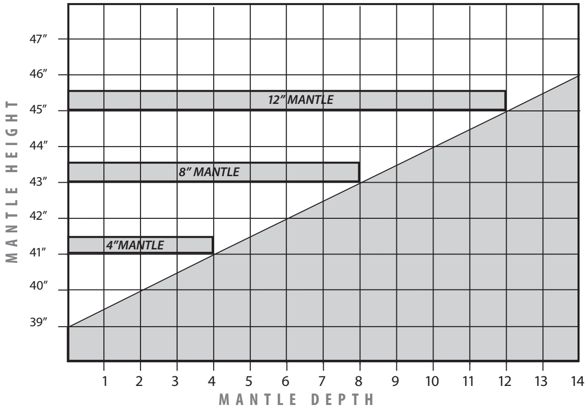
Figure 35(a): Minimum Mantel Height Non CSS
