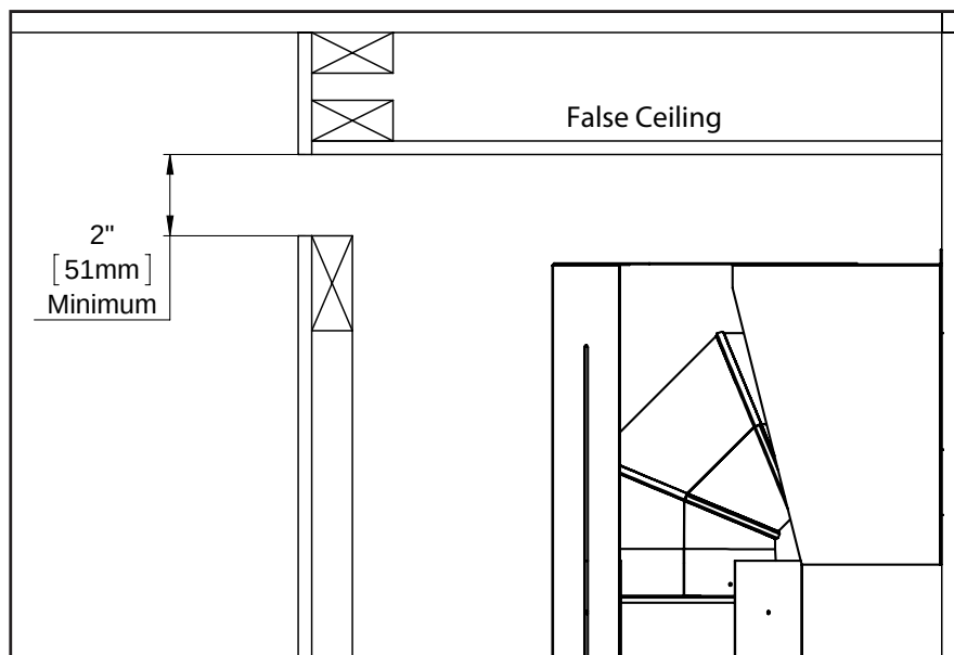
Figure 26: False Ceiling
